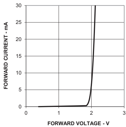
Figure 10: Forward Current vs. Forward Voltage Characteristics
