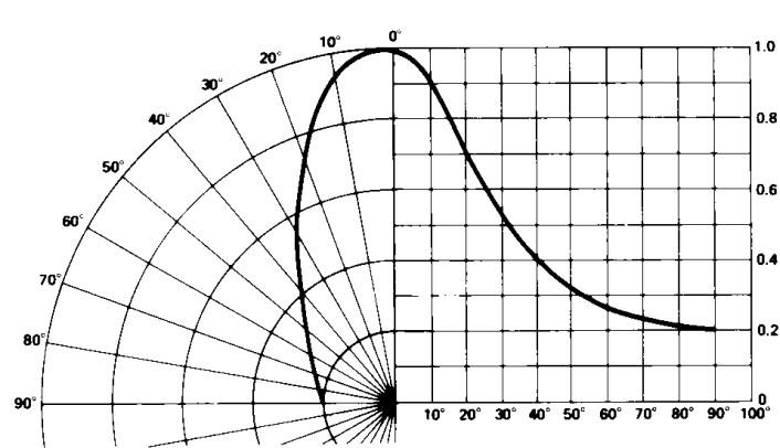
Figure 9: Relative Luminous Intensity vs. Angular Displacement
