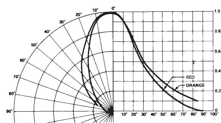
Figure 5: Relative Luminous Intensity vs. Angular Displacement
