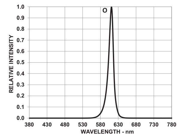
Figure 13: Relative Intensity vs. Wavelength
