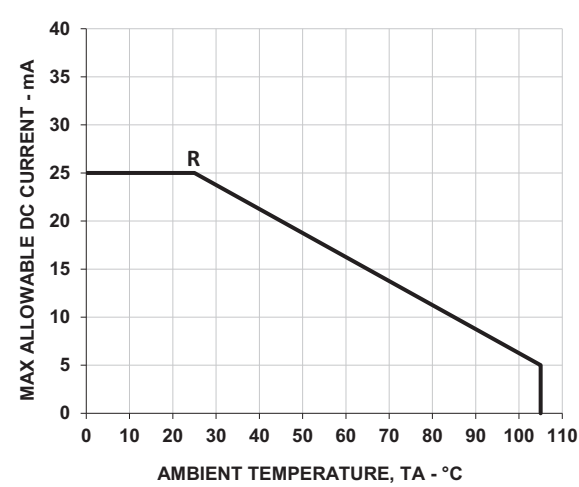
Figure 11: Allowable DC Current vs. Ambient Temperature
