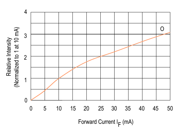
Figure 14: Relative Intensity vs. Forward Current
