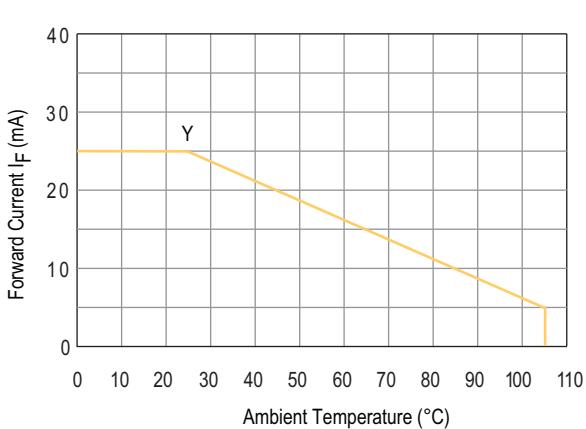
Figure 7: Allowable DC Current vs. Ambient Temperature
