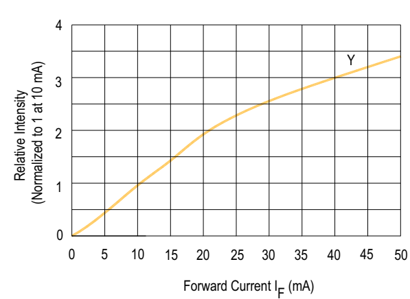
Figure 6: Relative Intensity vs. Forward Current
