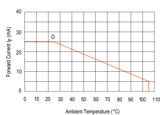
Figure 15: Allowable DC Current vs. Ambient Temperature
