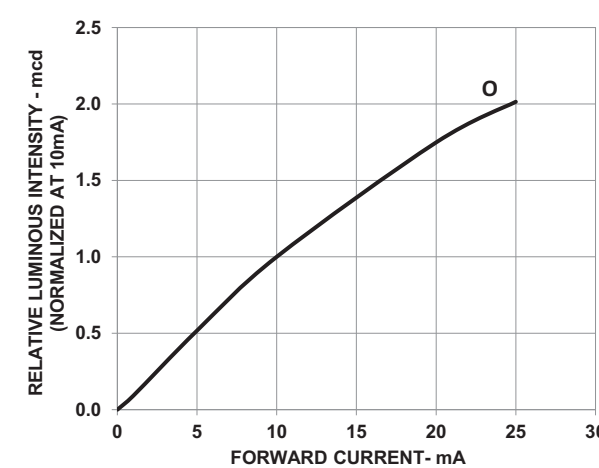
Figure 14: Relative Intensity vs. Forward Current
