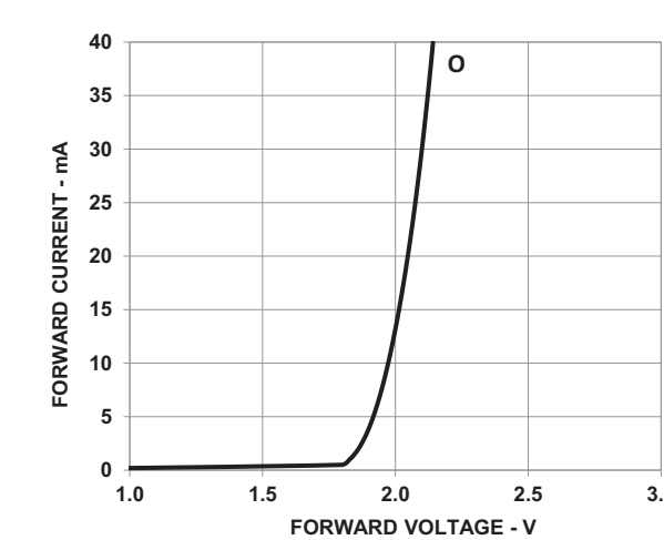
Figure 16: Forward Current vs. Forward Voltage
