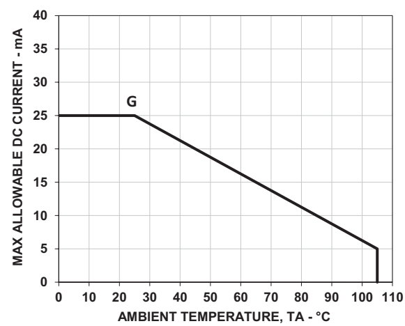
Figure 3: Allowable DC Current vs. Ambient Temperature
