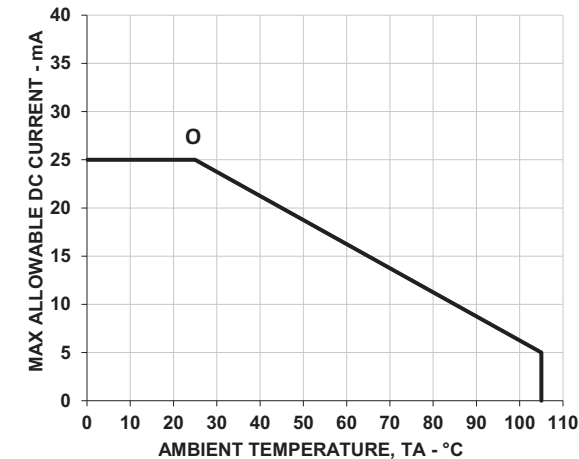
Figure 15: Allowable DC Current vs. Ambient Temperature
