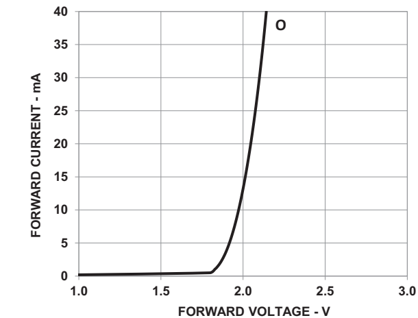
Figure 16: Forward Current vs. Forward Voltage
