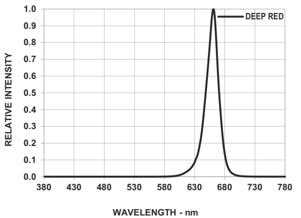
Figure 9: Spectral Power Distribution
