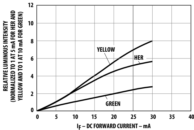
Figure 5: Relative Luminous Intensity vs. DC Forward Current
