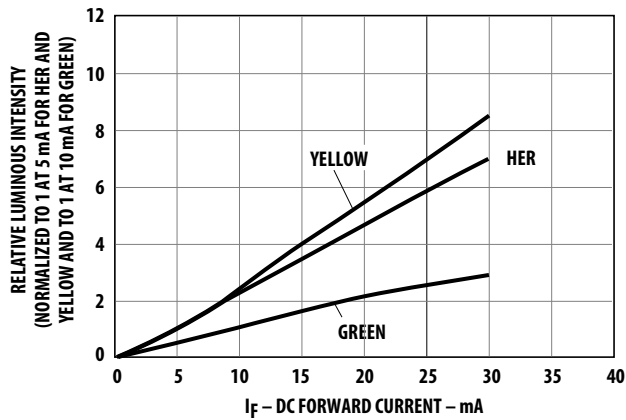
Figure 8: Relative Luminous Intensity vs. DC Forward Current
