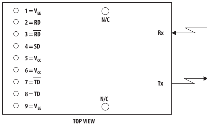
Figure 5: Pinout Diagram
