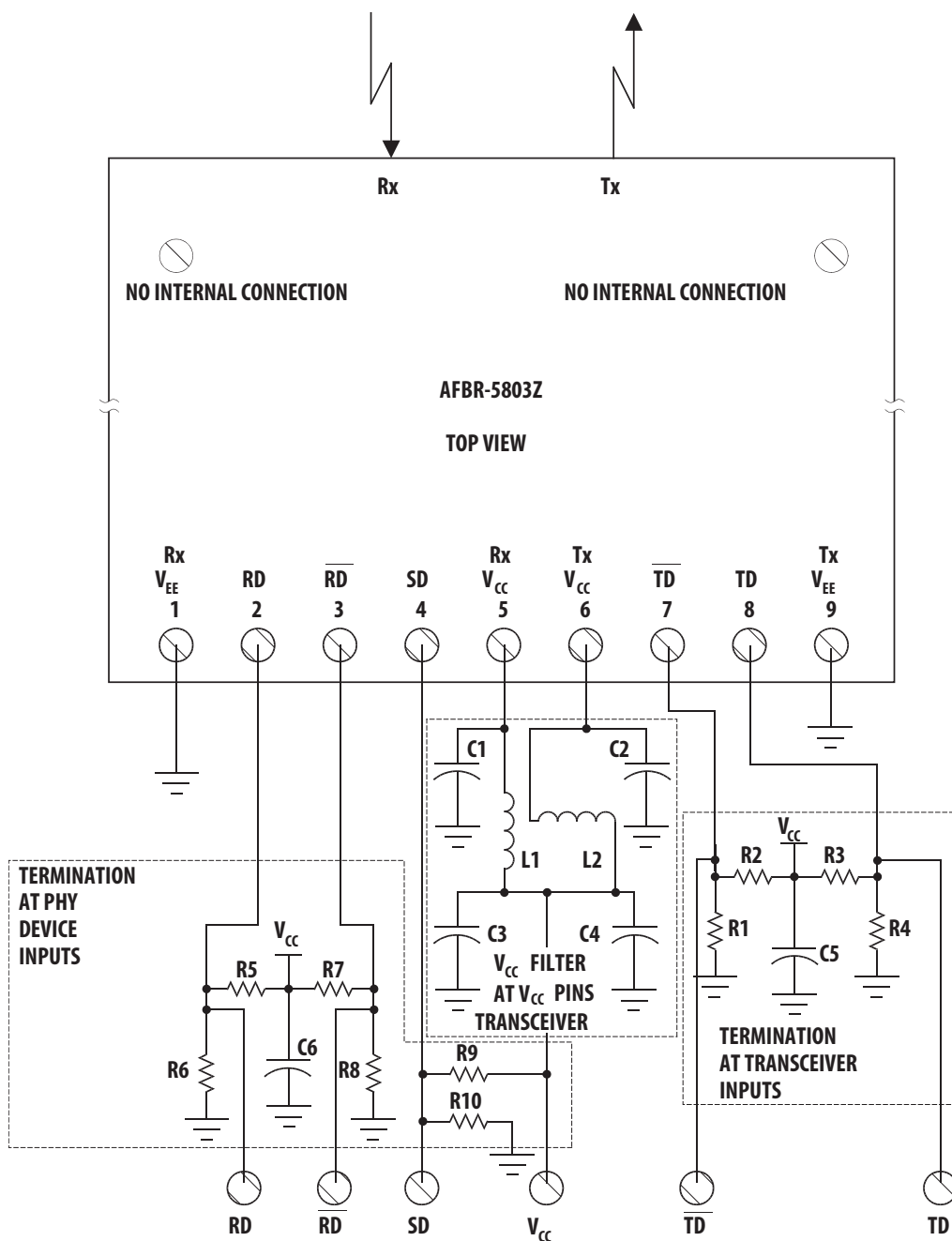
Figure 9: Recommended Decoupling and Termination Circuits
