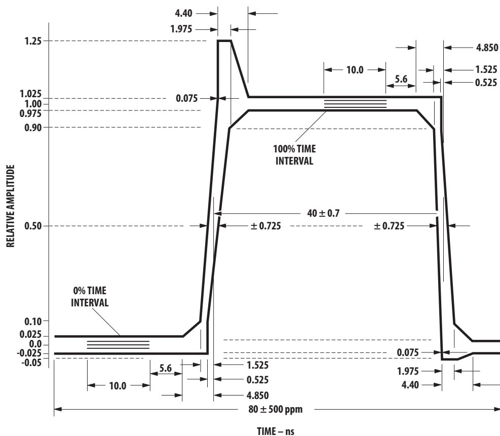
Figure 13: Output Optical Pulse Envelope
