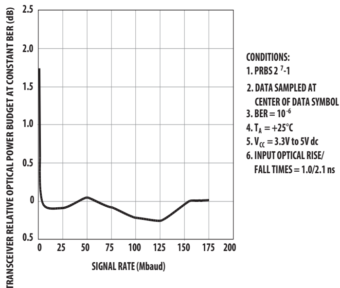
Figure 7: Transceiver Relative Optical Power Budget at Constant BER vs. Signaling Rate
