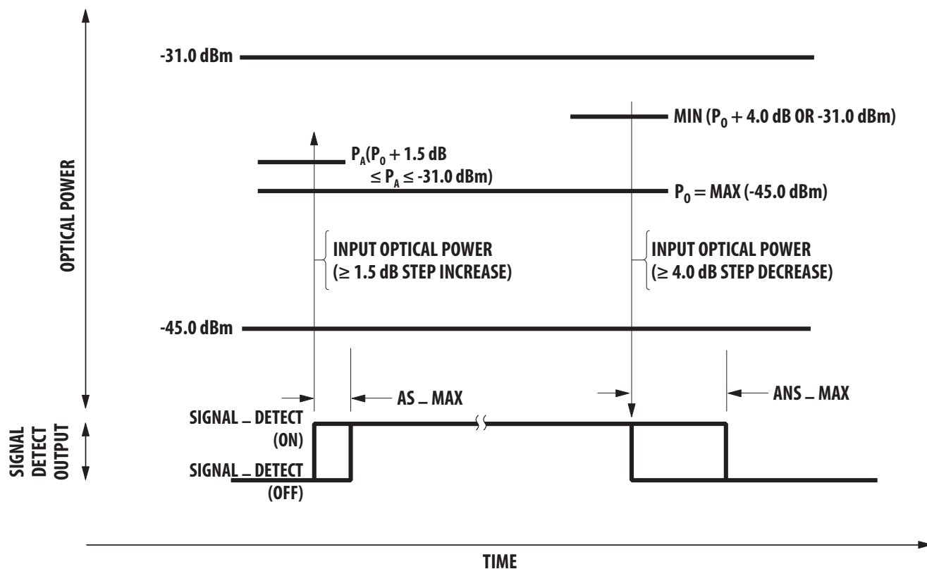
Figure 15: Signal Detect Thresholds and Timing
