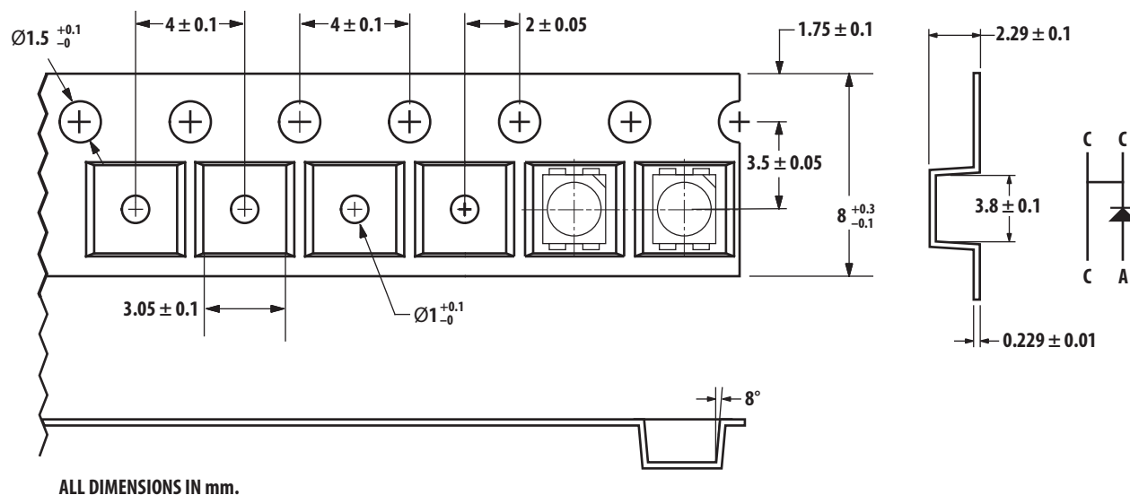
Figure 11: Reeling Orientation
