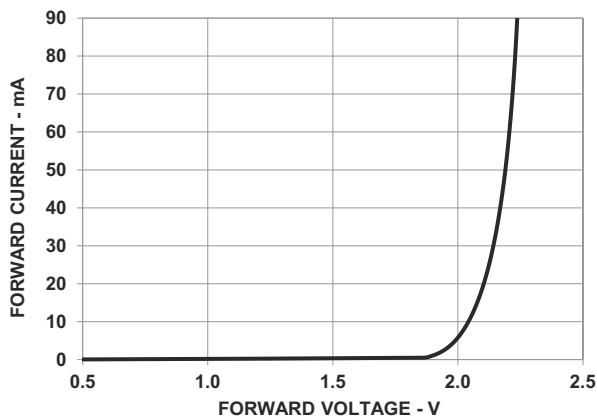
Figure 11: Forward Current vs. Forward Voltage
