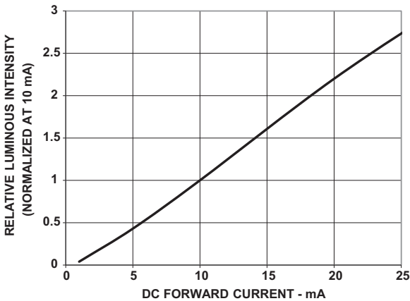
Figure 12: Relative Luminous Intensity vs. Forward Current
