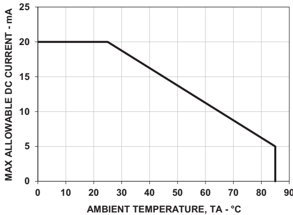
Figure 9: Maximum Forward Current vs. Ambient Temperature
