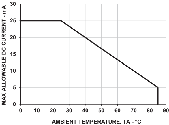
Figure 13: Maximum Forward Current vs. Ambient Temperature
