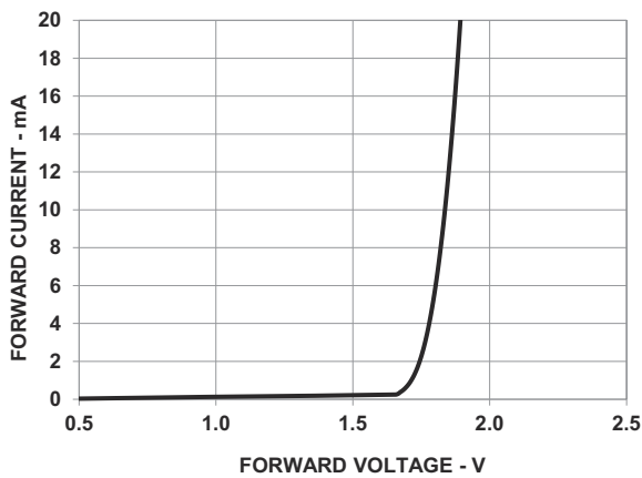
Figure 7: Forward Current vs. Forward Voltage
