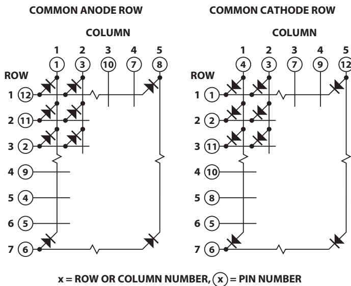
Figure 1: Common Anode and Cathode Rows
