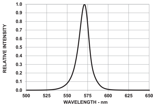
Figure 10: Relative Intensity vs. Wavelength
