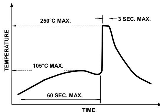
Figure 14: Recommended Wave Soldering Profile
