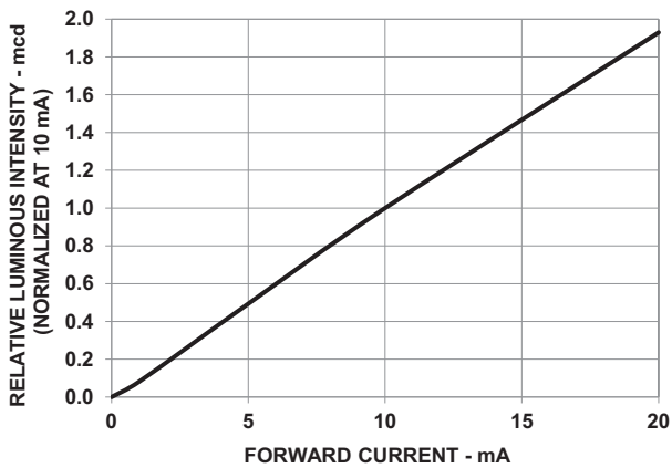
Figure 8: Relative Luminous Intensity vs. Forward Current
