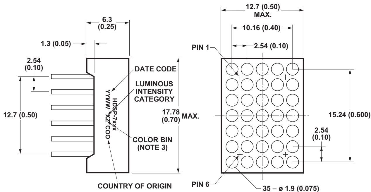
Figure 1: Package Drawing
