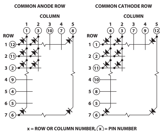
Figure 2: Common Anode and Cathode Rows
