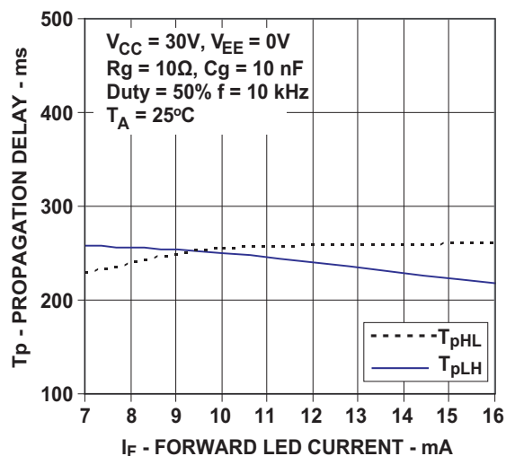
Figure 12: Propagation Delay vs. I_F
