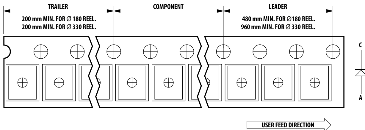
Figure 12: Tape Dimensions
