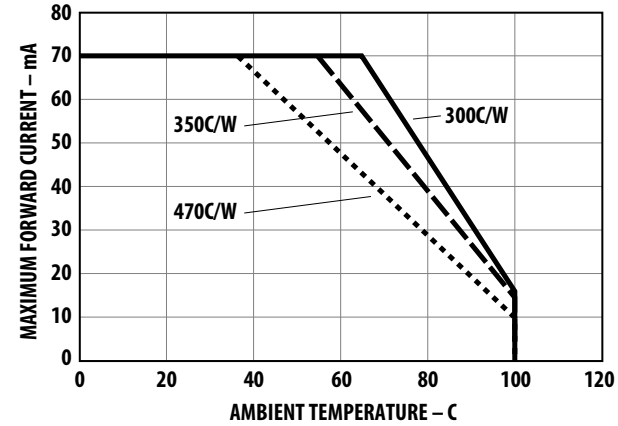
Figure 5: Maximum Forward Current vs. Ambient Temperature. Derated Based on TJmax = 110 °C (AlInGaP)
