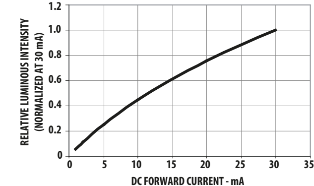
Figure 4: Relative Intensity vs. Forward Current (InGaP)
