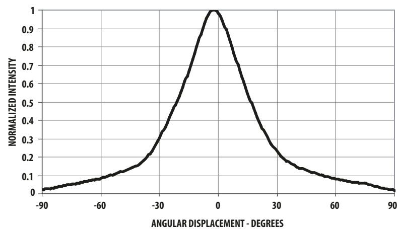
Figure 7: Radiation Pattern
