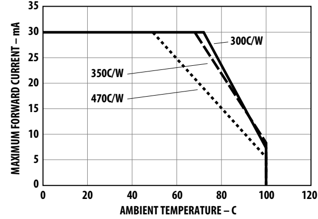
Figure 6: Maximum Forward Current vs. Ambient Temperature. Derated Based on TJmax = 110 °C (InGaP)
