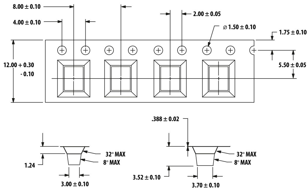
Figure 12: Tape Dimensions
