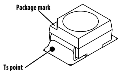
Figure 18: Solder Point Temperatures on PCB
