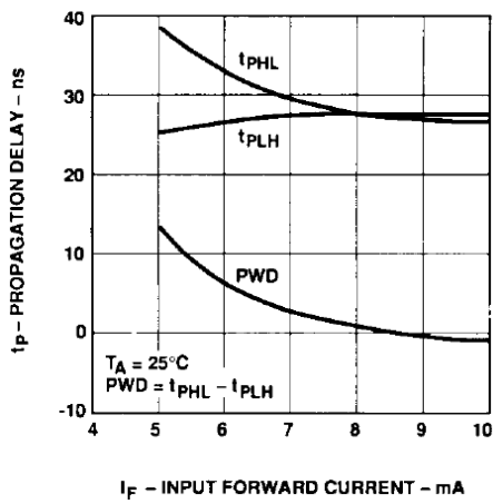
Figure 7 Typical Propagation Delay vs. Input Forward Current
