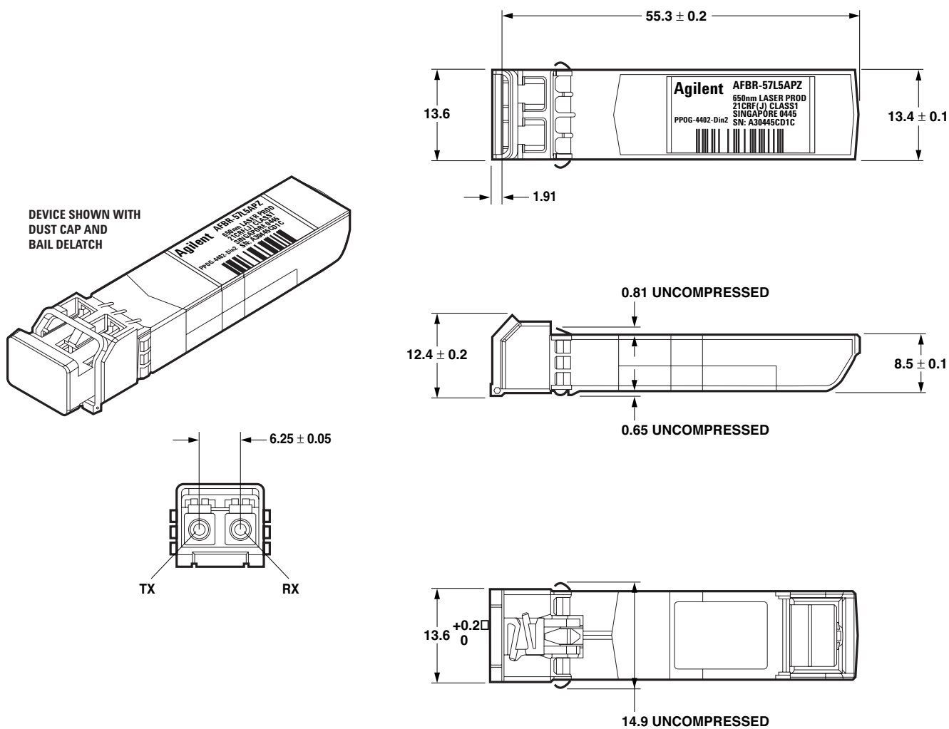
Figure 5. Module drawing.
