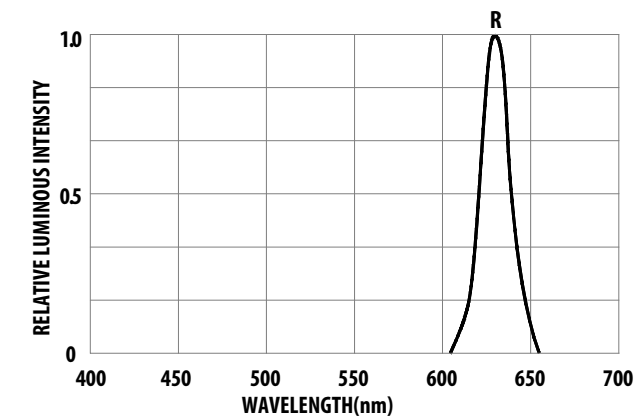
Figure 9: Relative Luminous Intensity vs. Wavelength
