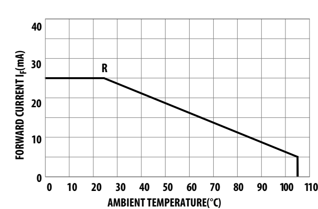
Figure 11: Allowable DC Current vs. Ambient Temperature
