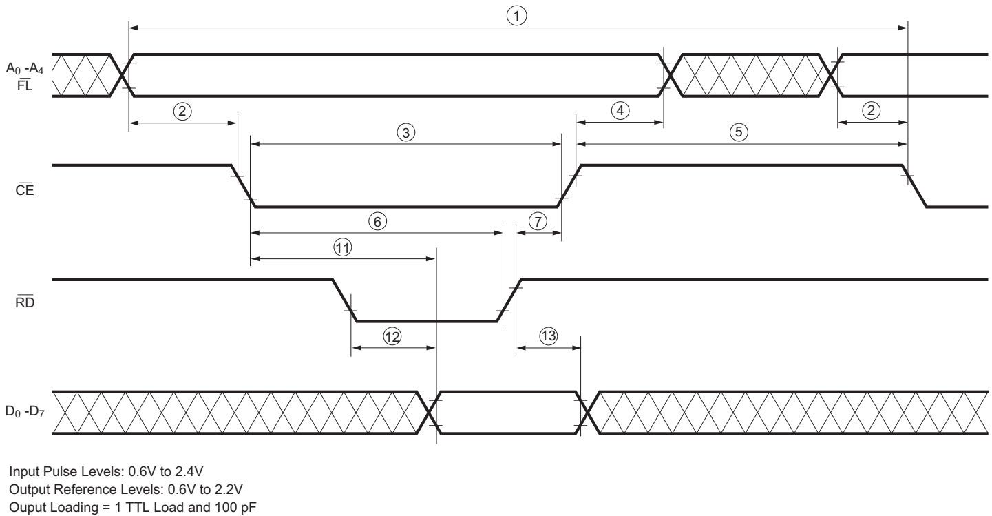
Figure 4: Read Cycle Timing Diagram
