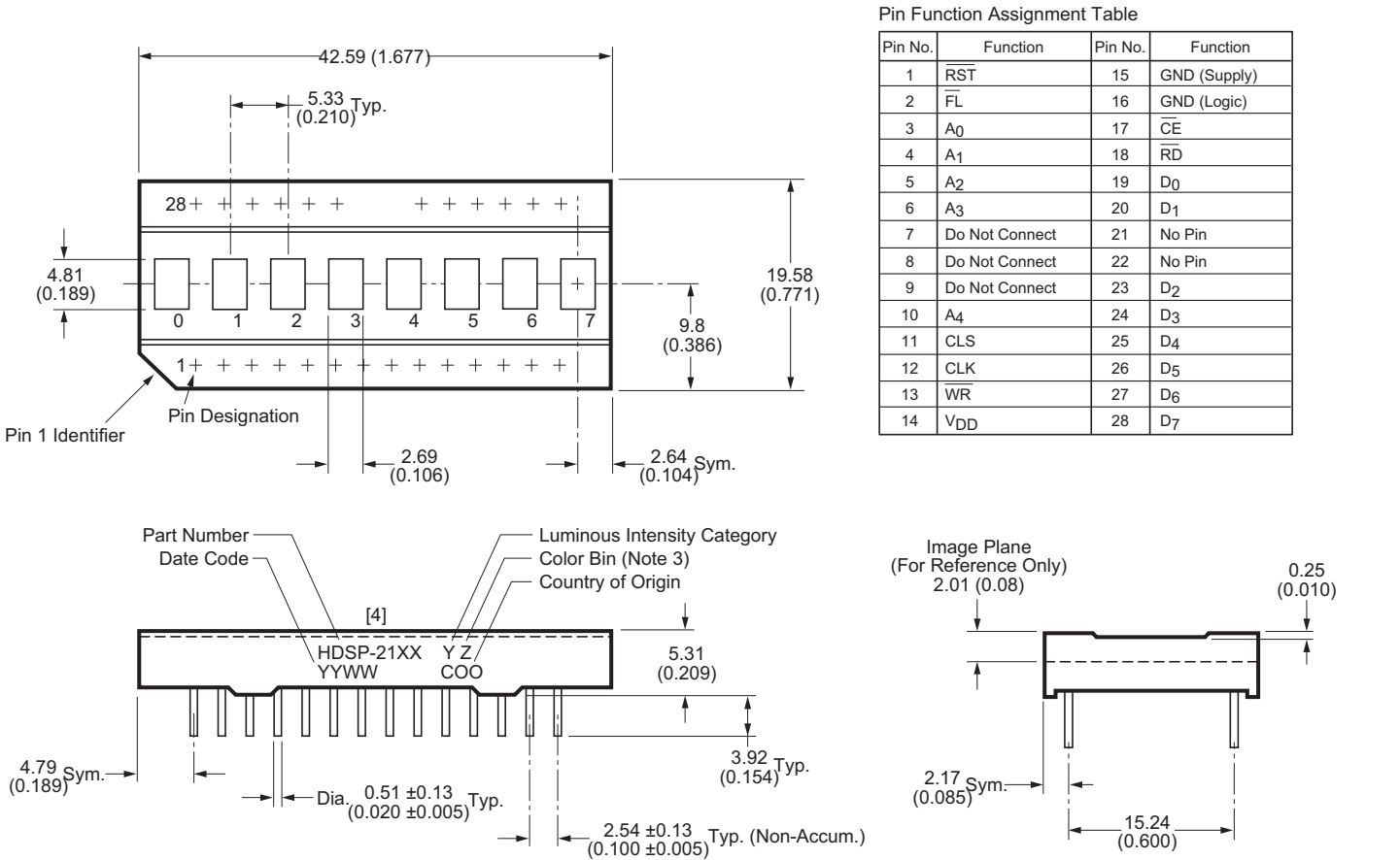
Figure 1: HDSP-21XX Package Dimensions
