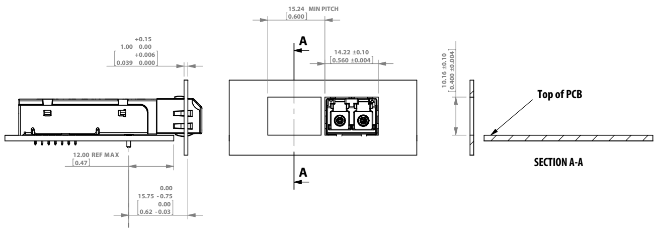
Figure 7. Assembly Drawing
