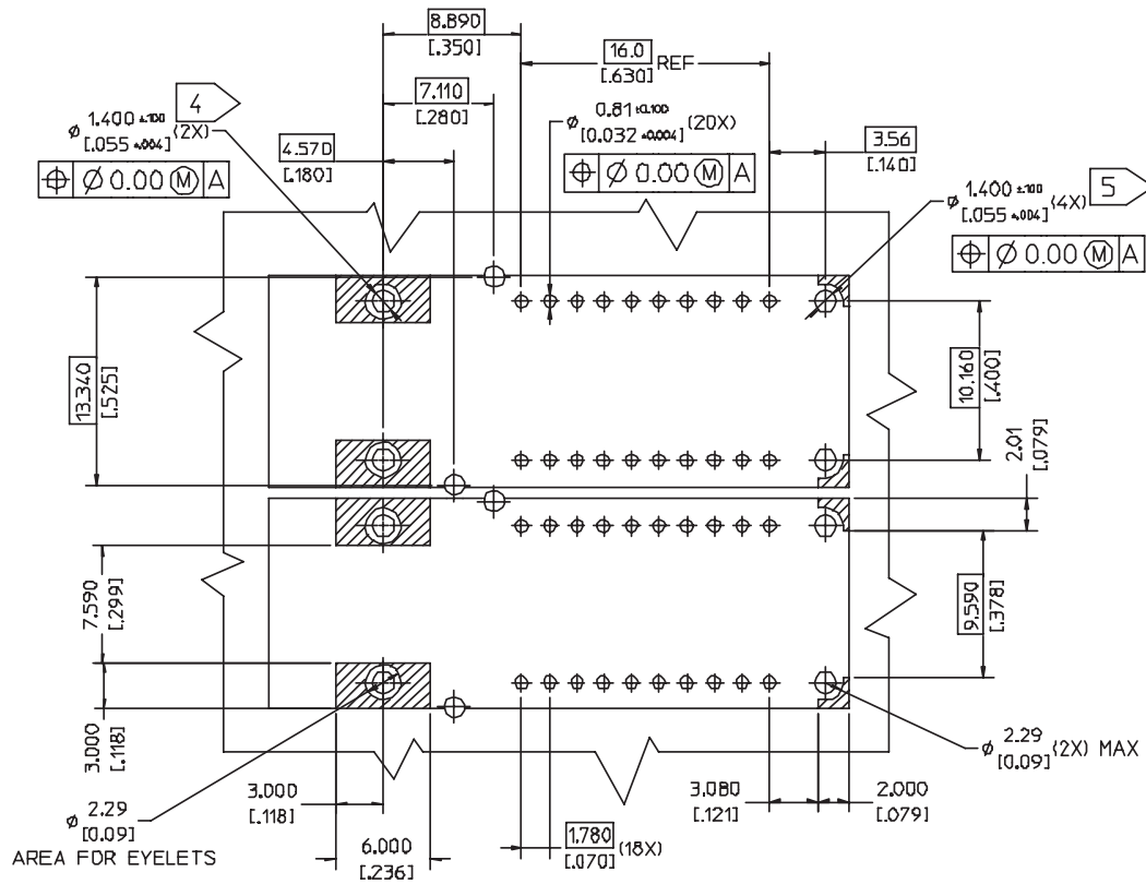
Figure 8. Board Layout
