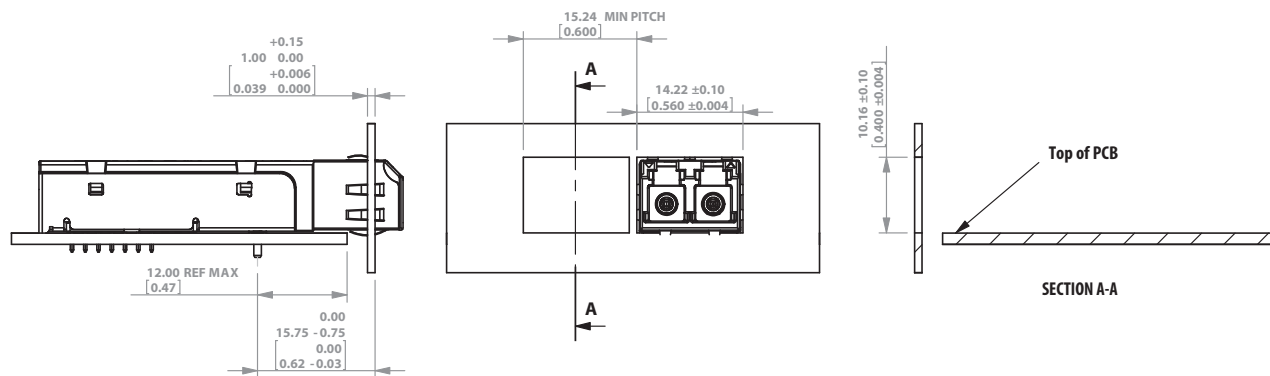
Figure 7. Assembly Drawing
