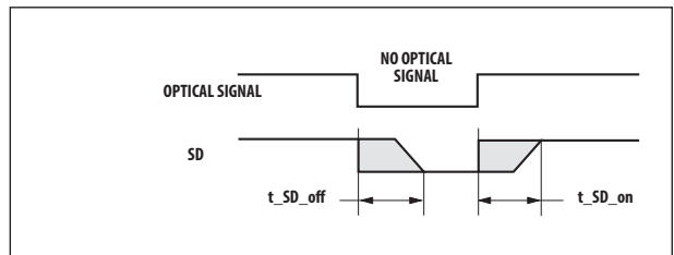
t_{\text{SD\_off}} & t_{\text{SD\_on}}
