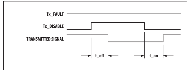
t_{\text{off}} & t_{\text{on}} : TX DISABLE ASSERTED THEN NEGATED
