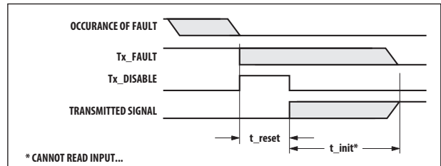
t_{\text{reset}} : TX DISABLE ASSERTED THEN NEGATED, TX SIGNAL RECOVERED
