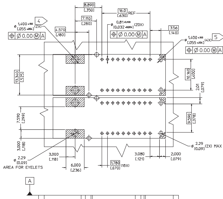
Figure 7. Assembly Drawing
