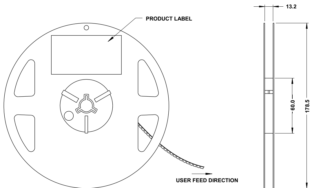
Figure 19: Reel Dimensions
