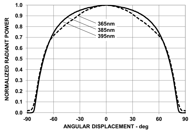
Figure 10: Radiation Pattern – 130°
