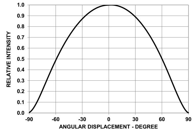
Figure 7: Radiation Pattern
