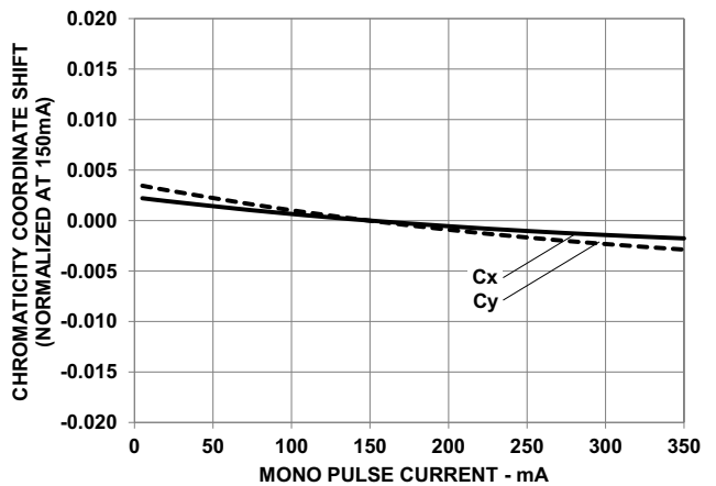
Figure 8: Chromaticity Coordinate Shift vs. Mono Pulse Current – 3000K
