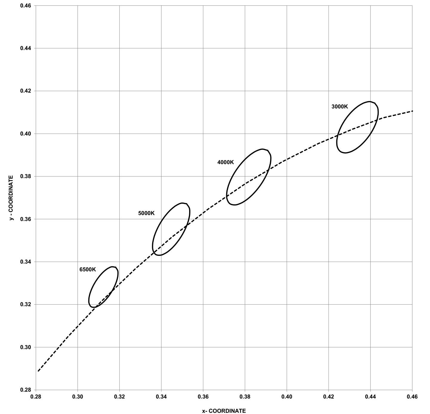
Figure 3: Chromaticity Diagram
