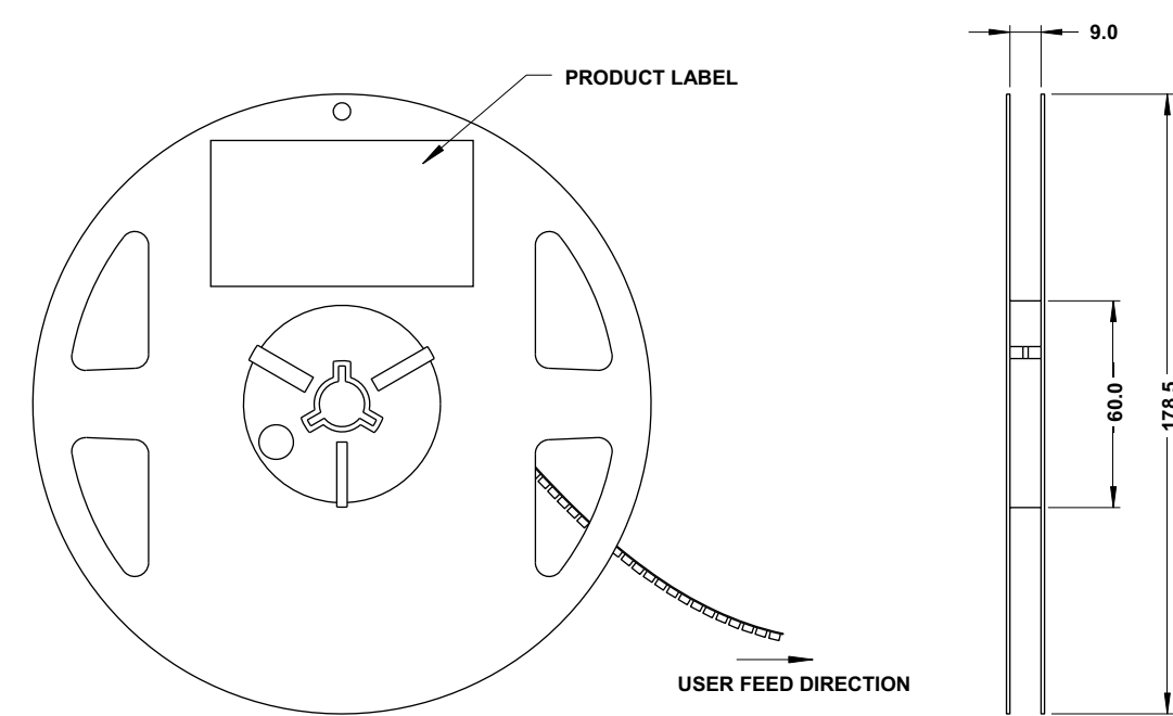
Figure 22: Reel Dimensions
