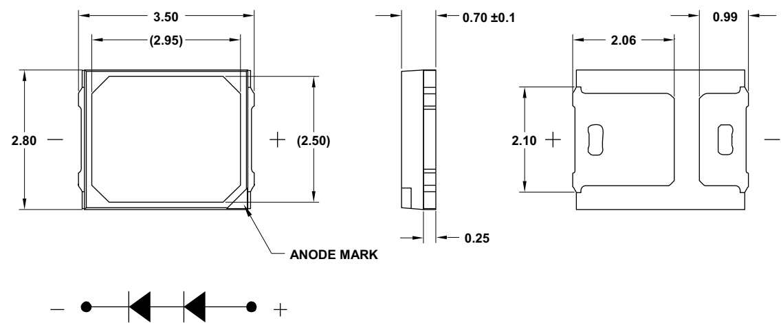
Figure 1: Package Drawing
