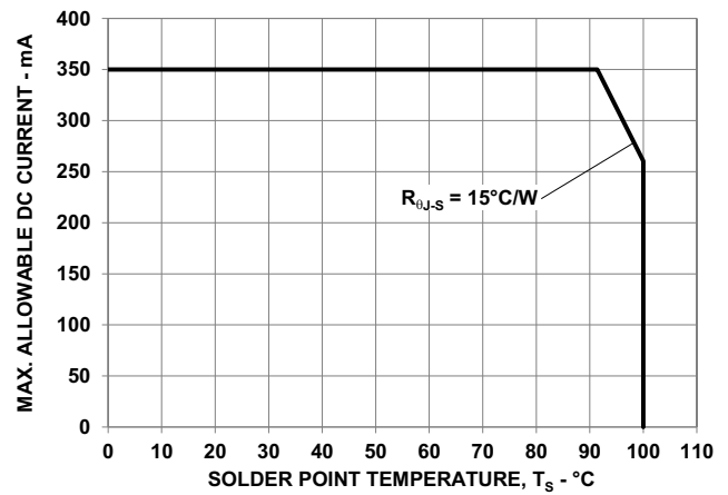
Figure 19: Maximum Forward Current vs. Solder Point Temperature. Derated based on T_{JMAX} = 125^{\circ}\text{C} , R_{\theta J-S} = 15^{\circ}\text{C/W}
