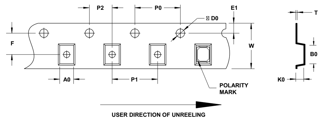
Figure 21: Carrier Tape Dimensions
