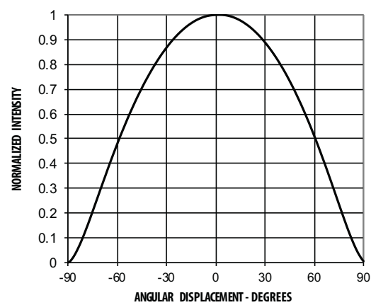
Figure 15 Radiation Pattern
