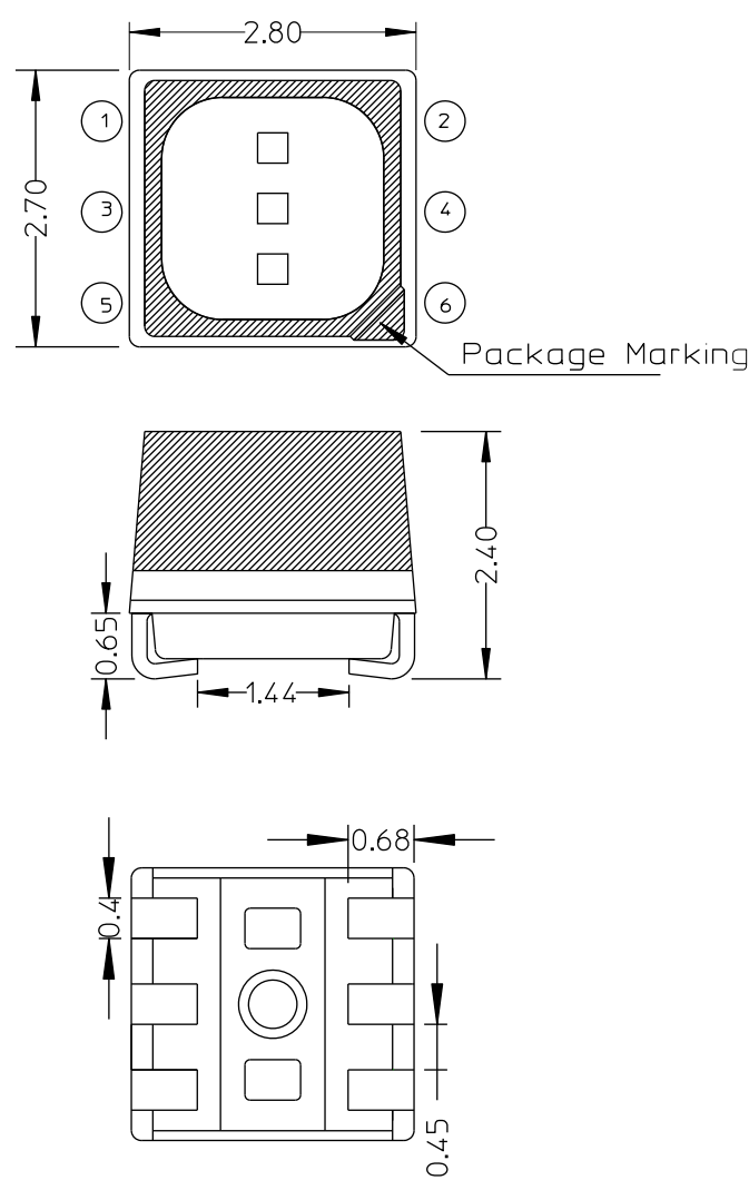
Figure 1: Package Drawing
