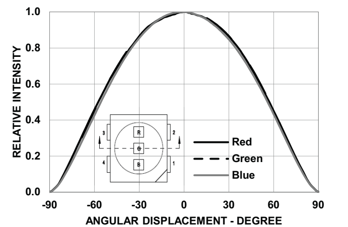
Figure 10: Radiation Pattern for X-axis
