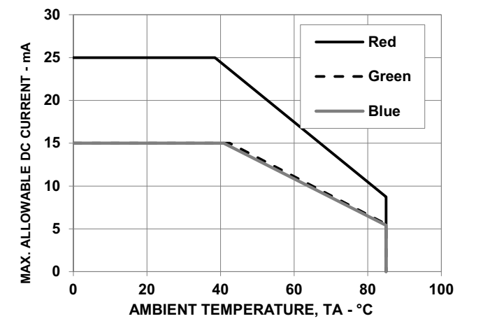
Figure 8: Maximum Forward Current vs. Temperature for Red, Green, and Blue
