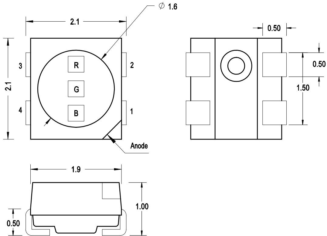
Figure 1: Package Drawing
