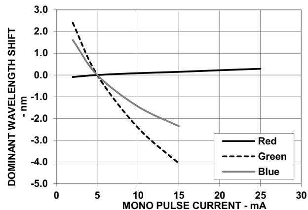
Figure 5: Dominant Wavelength Shift vs. Mono Pulse Current
