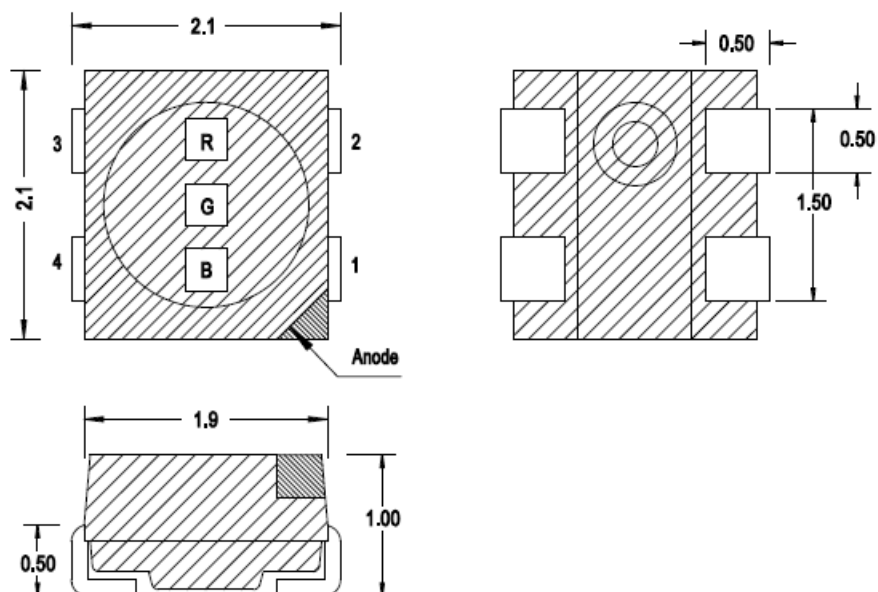
Figure 1: Package Drawing
