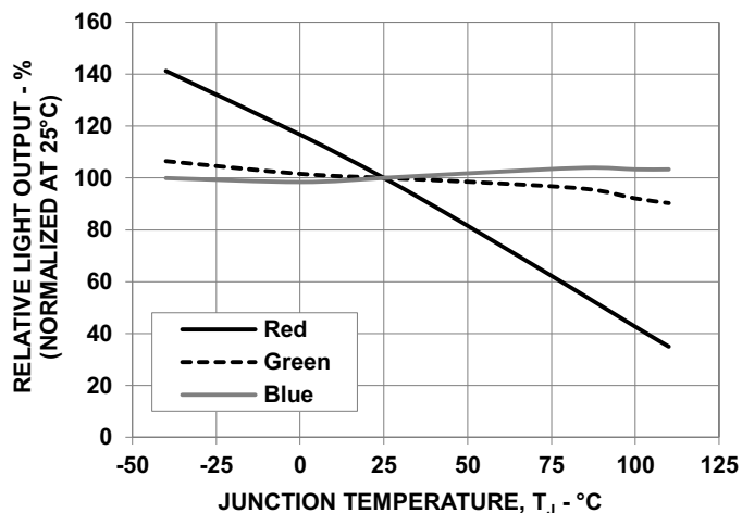
Figure 6: Relative Light Output vs. Junction Temperature
