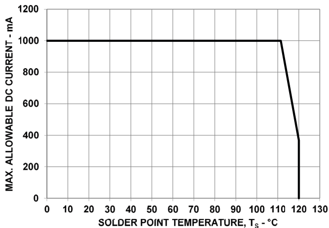
Figure 20: Maximum Forward Current vs. Solder Point Temperature
