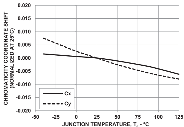
Figure 18: Chromaticity Coordinate Shift vs. Junction Temperature – 6500K
