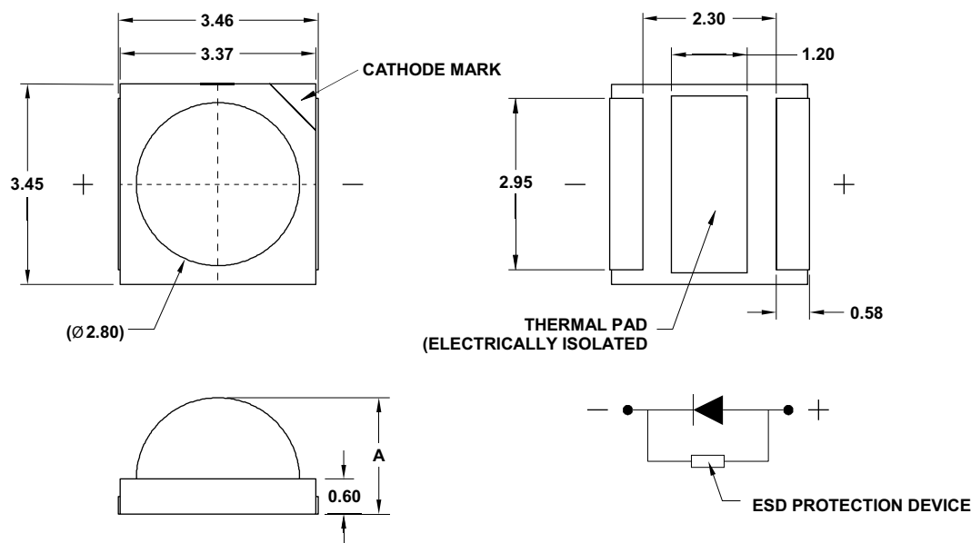
Figure 1: Package Drawing
