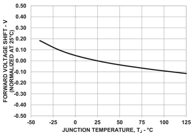
Figure 14: Forward Voltage Shift vs. Junction Temperature
