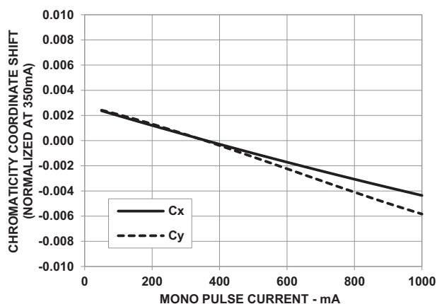
Figure 12: Chromaticity Coordinate Shift vs. Mono Pulse Current – 6500K
