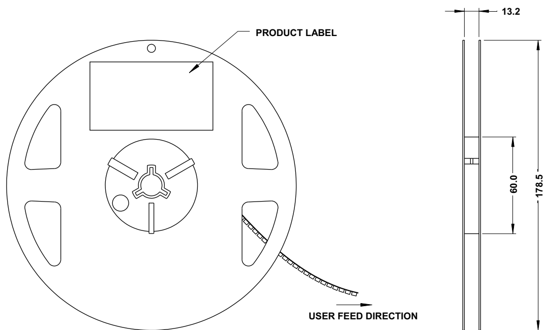
Figure 23: Reel Dimensions
