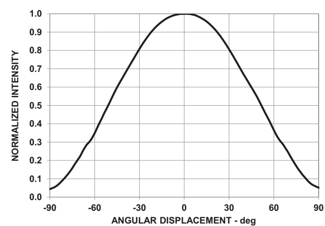
Figure 7: Radiation Pattern – 90°
