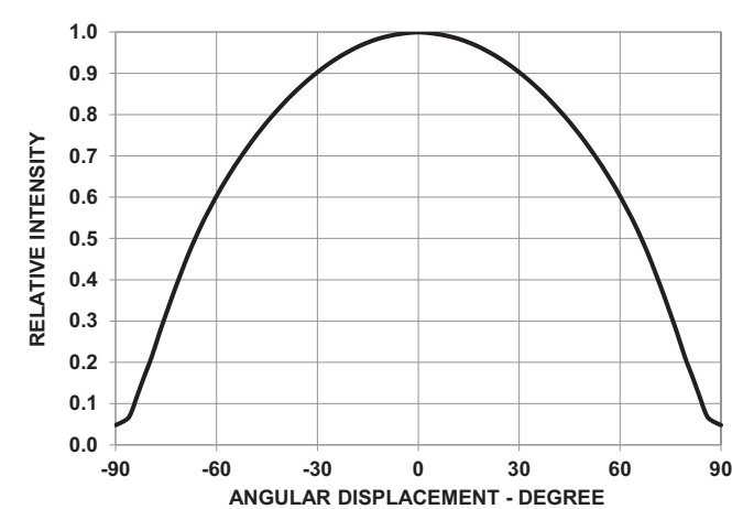
Figure 8: Radiation Pattern – 130°
