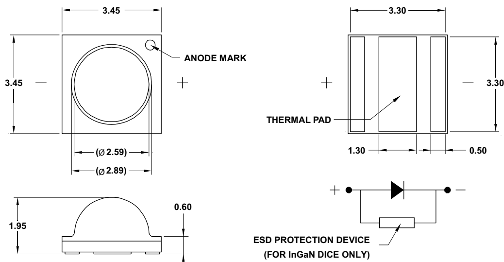
Figure 1: Package Drawing
