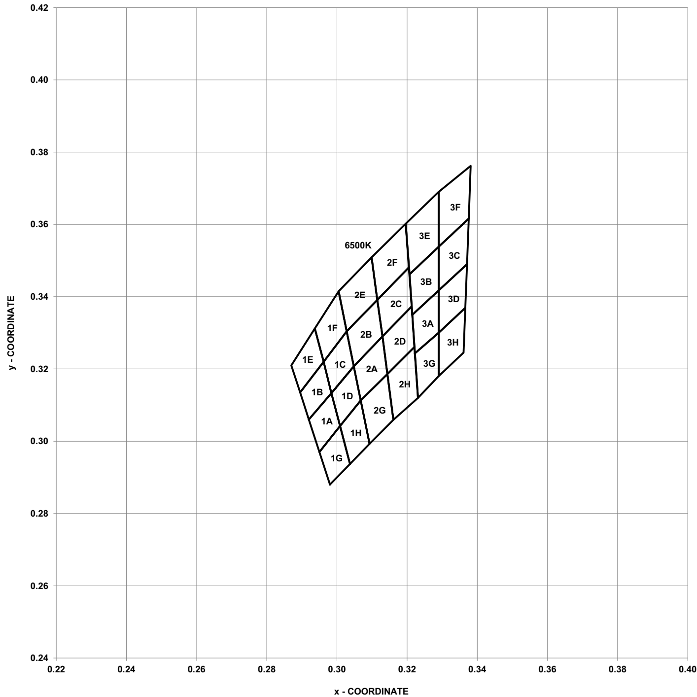
Figure 2: Chromaticity Diagram
