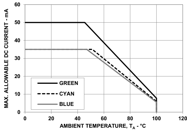
Figure 18: Maximum Forward Current vs. Ambient Temperature - Green, Cyan, and Blue
