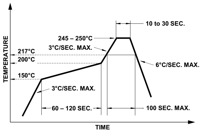
Figure 22: Recommended Lead-Free Reflow Soldering Profile
