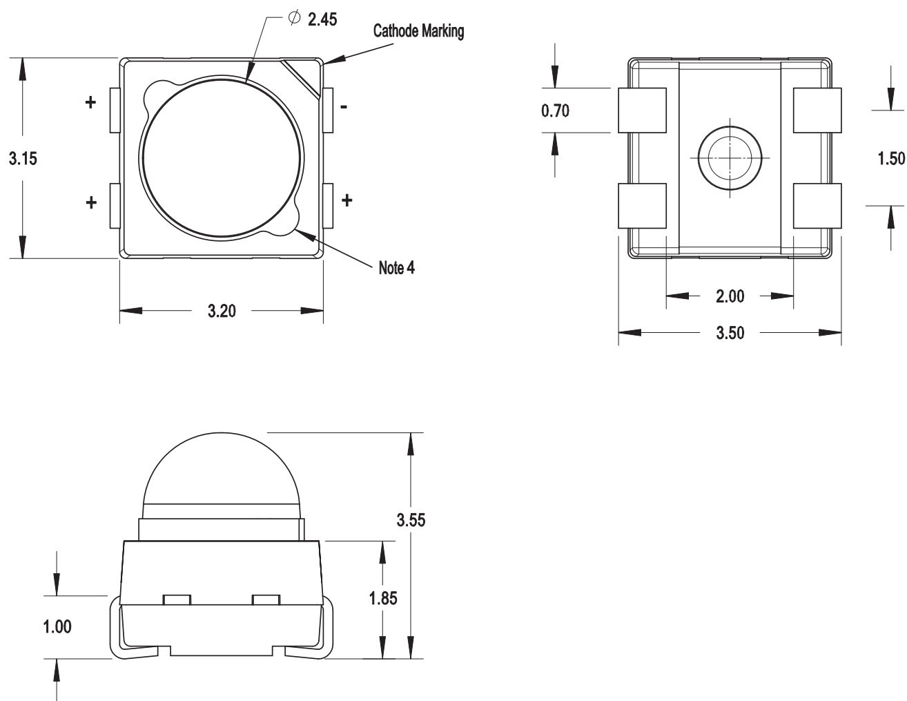
Figure 2: Package Drawing for White Surface ASCQDx30 Series
