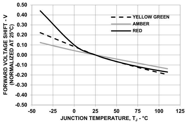
Figure 12: Forward Voltage Shift vs. Junction Temperature (AlInGaP)
