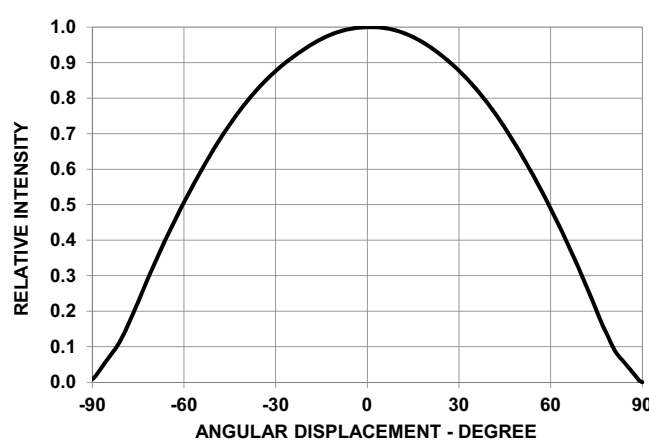
Figure 8: Radiation Pattern
