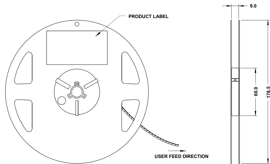
Figure 25: Reel Dimensions
