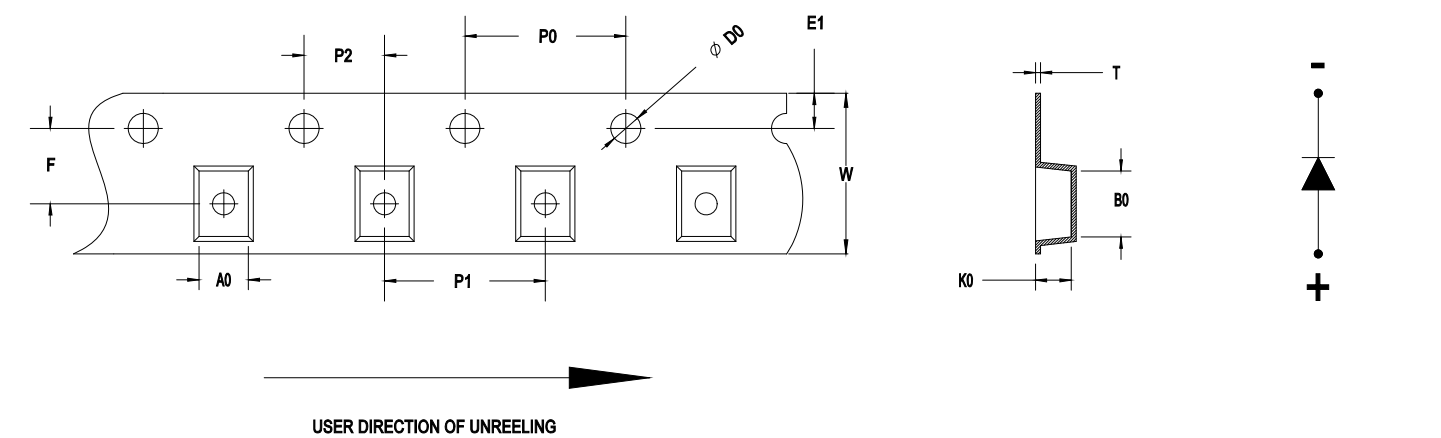
Figure 24: Carrier Tape Dimensions
