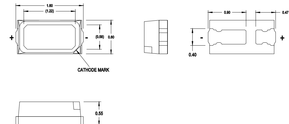
Figure 1: Package Drawing for Yellow-Green and Green
