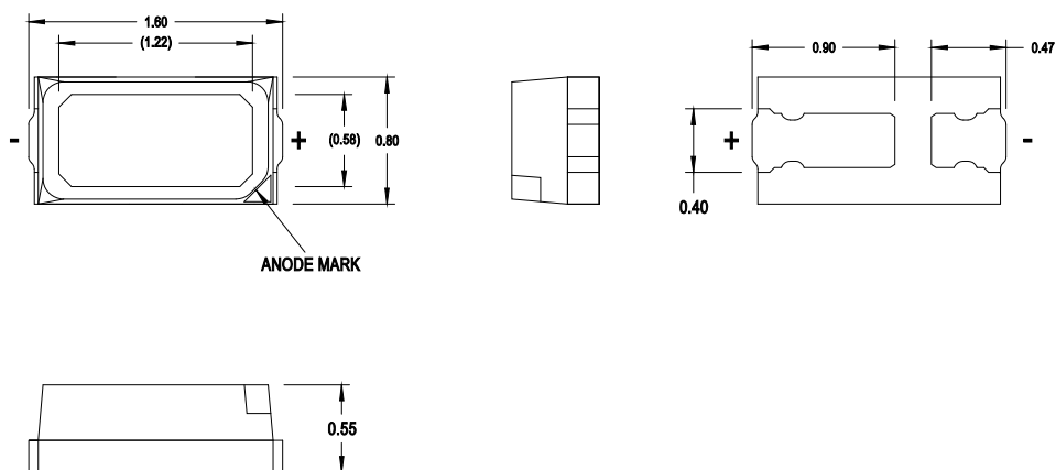
Figure 2: Package Drawing for Red, Amber, Blue, and PC Amber
