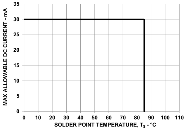
Figure 20: Maximum Forward Current vs. Solder Point Temperature. Derated Based on T_{JMAX} = 110^{\circ}\text{C} (AlInGaP)
