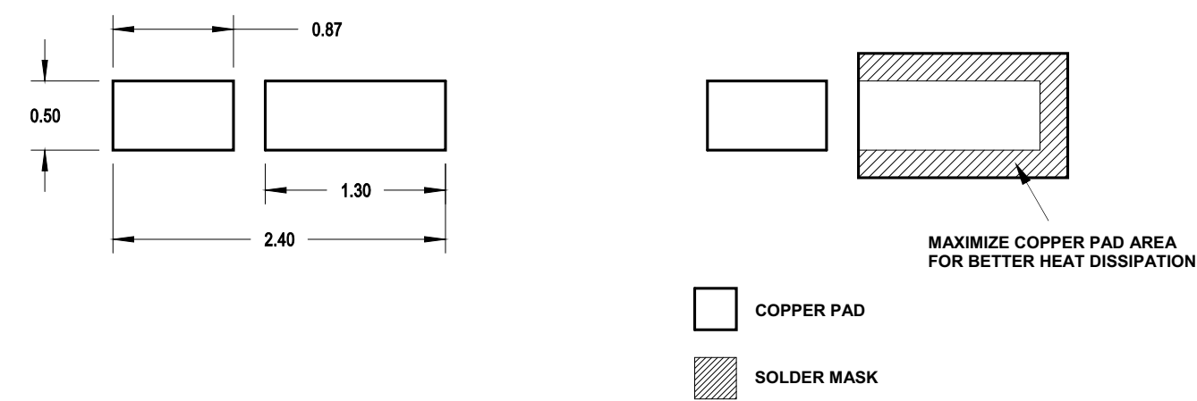
Figure 23: Recommended Soldering Land Pattern
