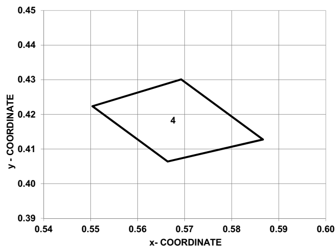
Figure 3: Chromaticity Diagram
