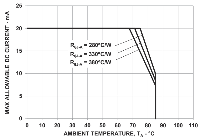
Figure 21: Maximum Forward Current vs. Ambient Temperature. Derated Based on T_{JMAX} = 95^{\circ}\text{C} (InGaN)
