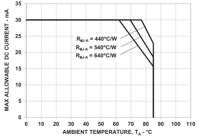
Figure 19: Maximum Forward Current vs. Ambient Temperature. Derated Based on T_{JMAX} = 110^{\circ}\text{C} (AlInGaP)
