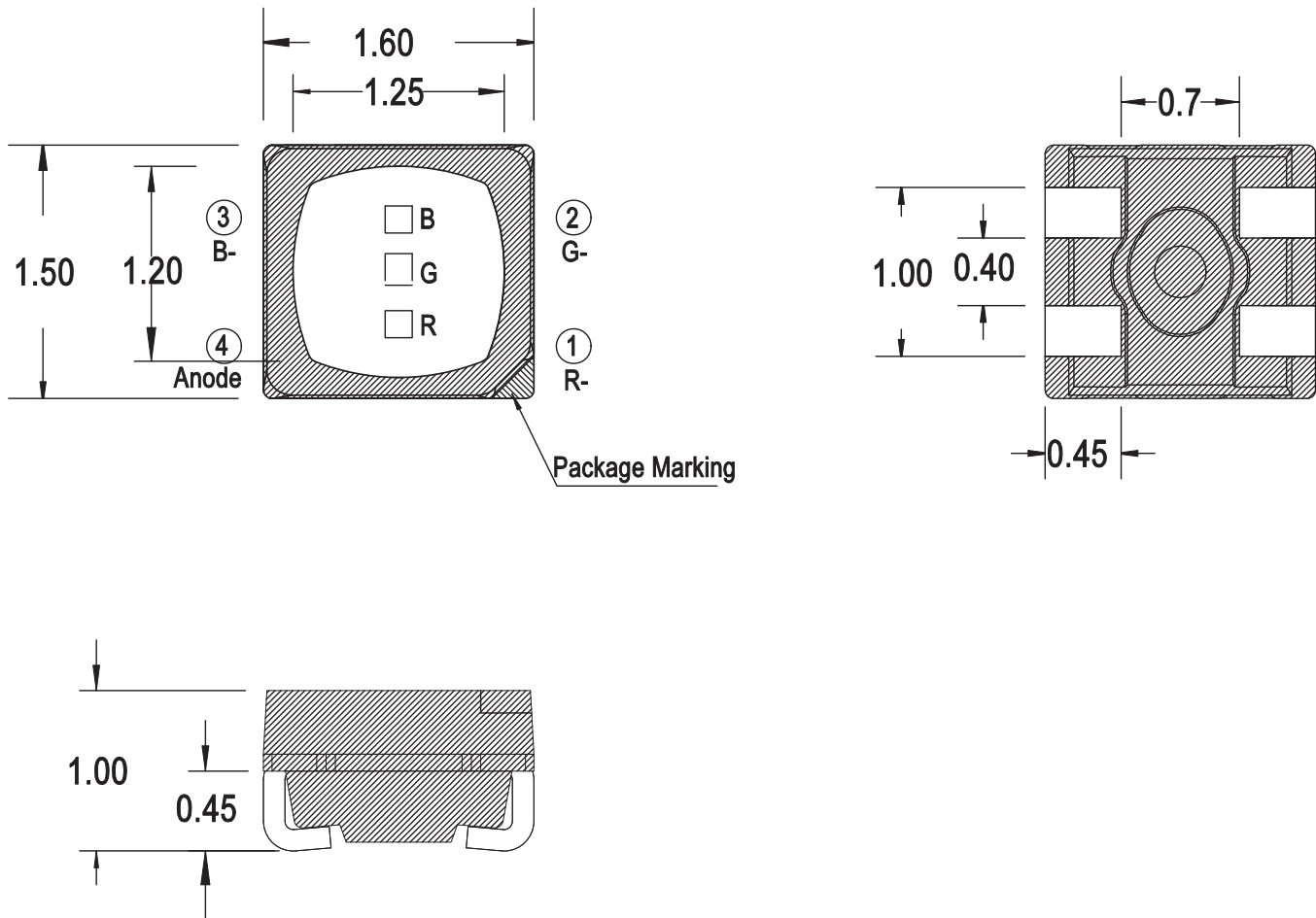
Figure 1: Package Drawing
