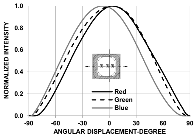
Figure 10: Radiation Pattern for y-axis
