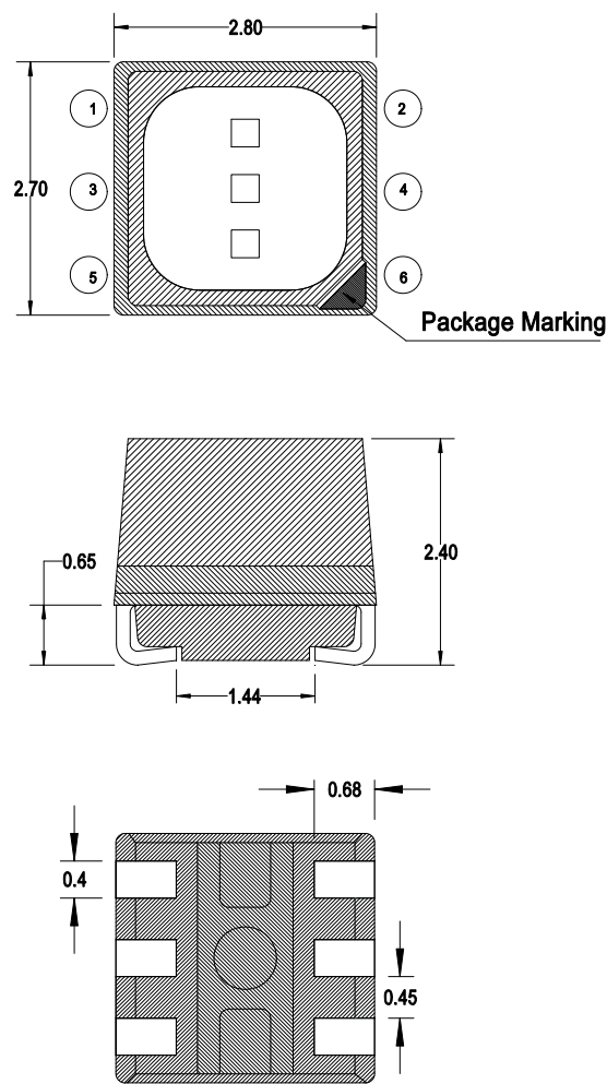
Figure 1: Package Drawing
