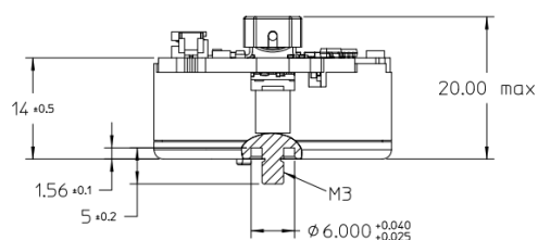
M3 Hub Screw
