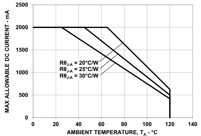
Figure 11: Maximum Forward Current vs. Ambient Temperature for ARE6-95D1
