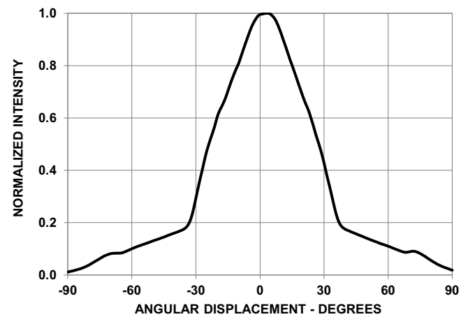
Figure 7: Radiation Pattern
