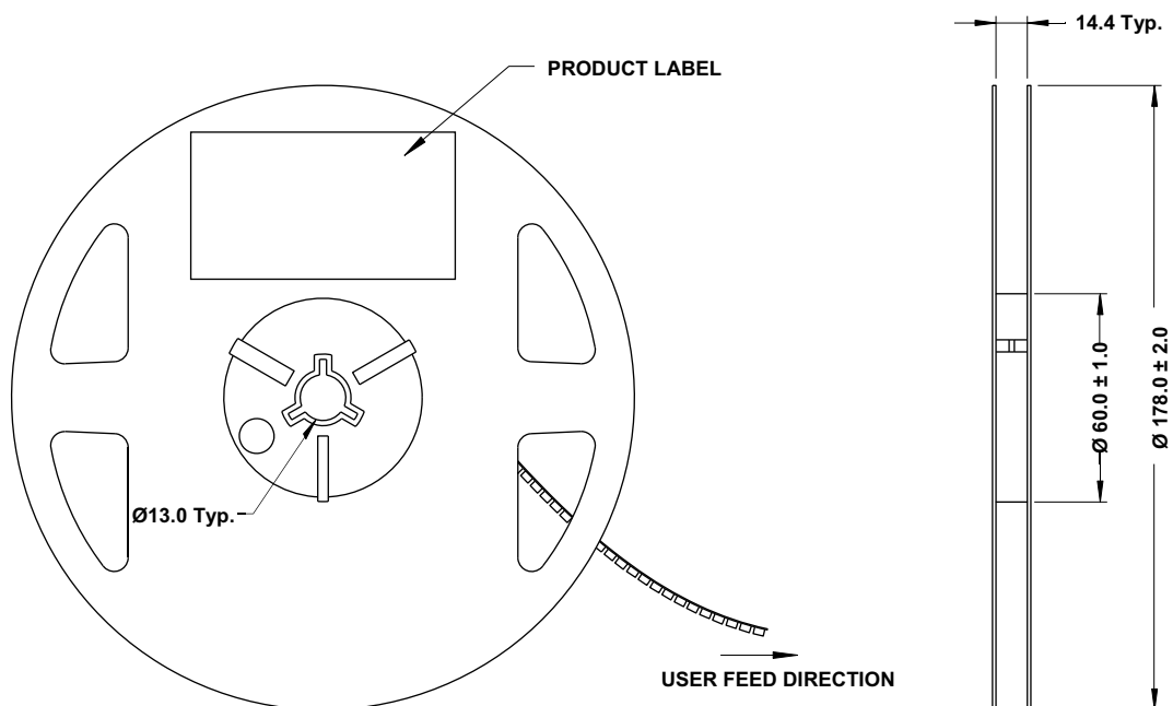
Figure 16: Reel Dimensions
