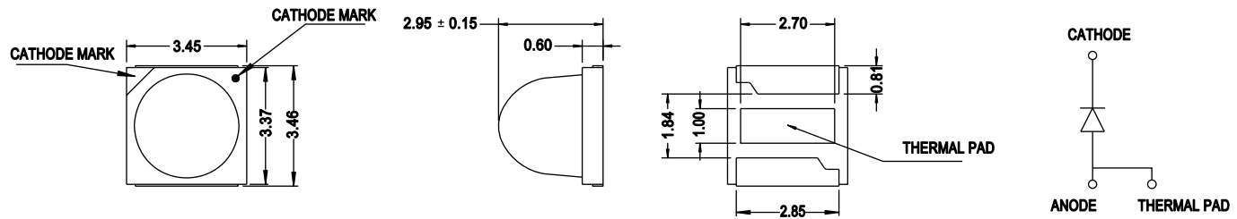
Figure 1: Package Drawing
