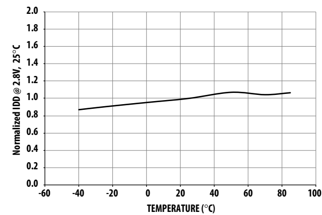
Figure 7: Normalized IDD vs. Temperature
