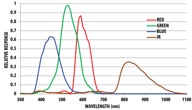
Figure 2: Normalized PD Spectral Response
