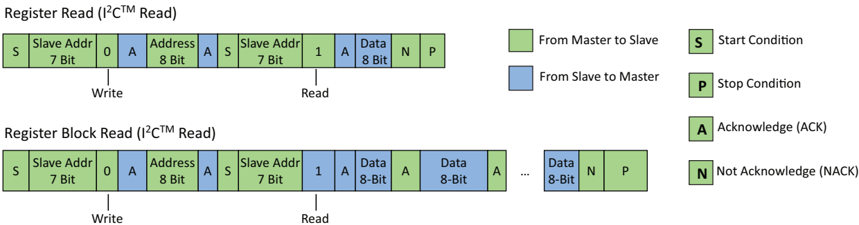
Figure 10: I 2 C Register Read Timing Diagram
