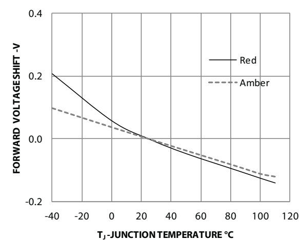
Figure 11: Forward Voltage shift vs. Junction Temperature
