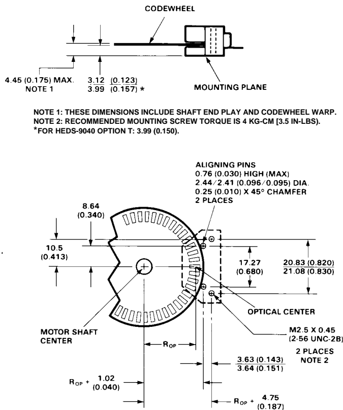
Figure 5. Mounting Plane Side A.
