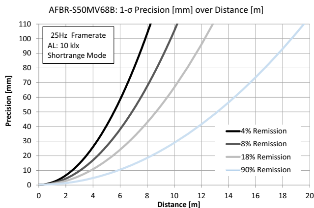
Figure 9: Typical Precision [mm] over Distance [m] – 10 klx, Short Range Mode
