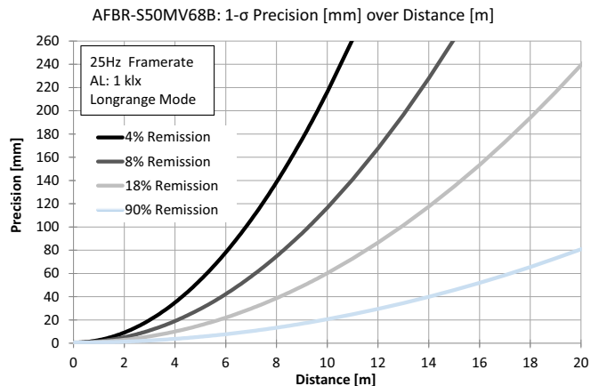
Figure 14: Typical Precision [mm] over Distance [m] – 1 klx, Long Range Mode
