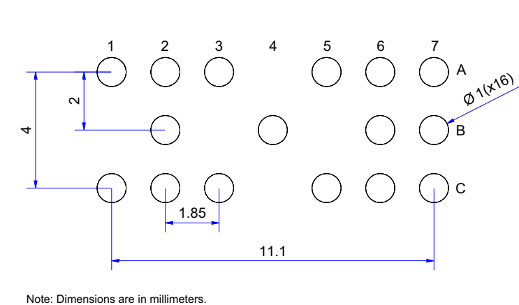
Figure 3: Recommended Landing Pattern Diagram
