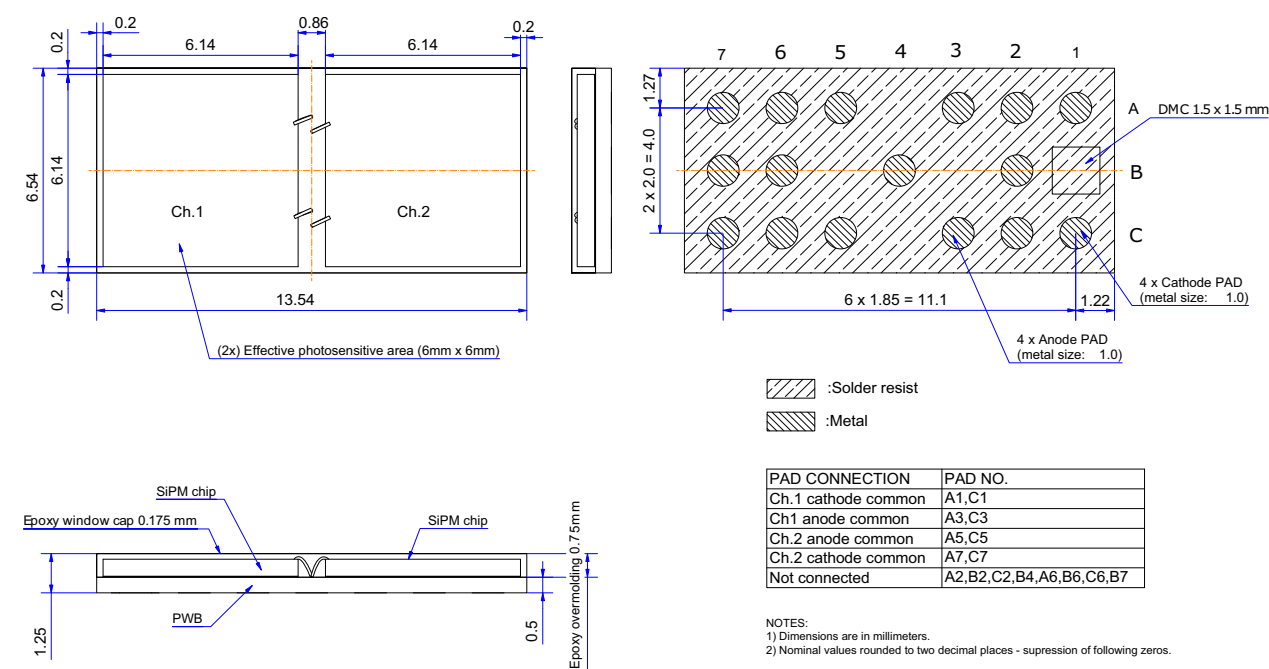
Figure 2: Package Drawing with Dimensions
