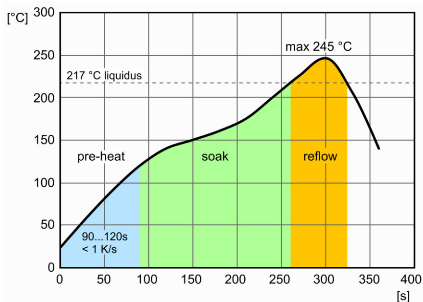
Figure 4: Recommended Reflow Soldering Profile
