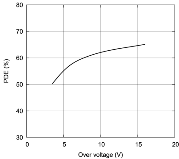
Figure 6: PDE at Peak λ vs. OV
