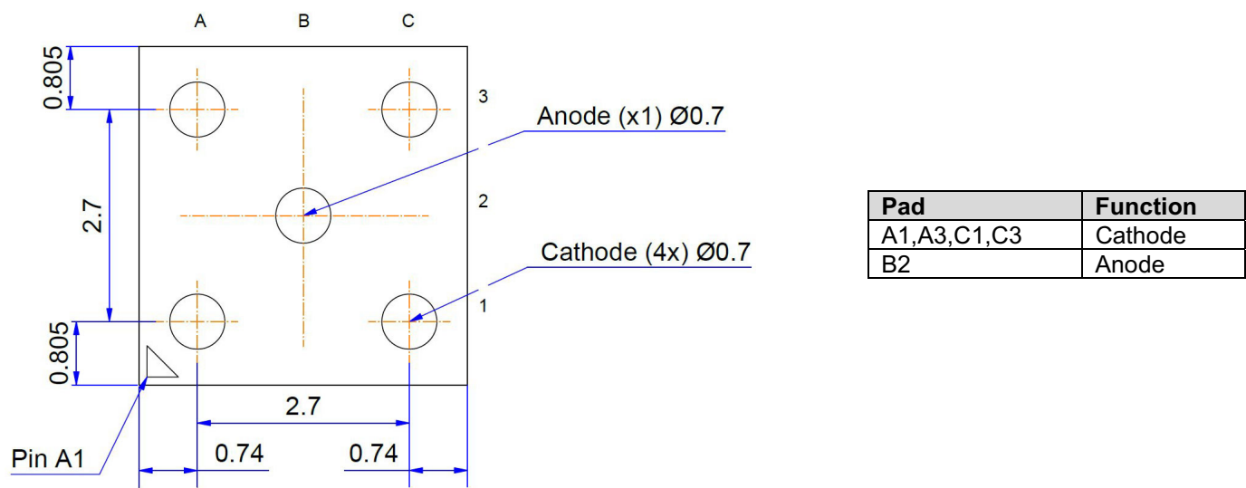
Figure 2: Pad Layout
