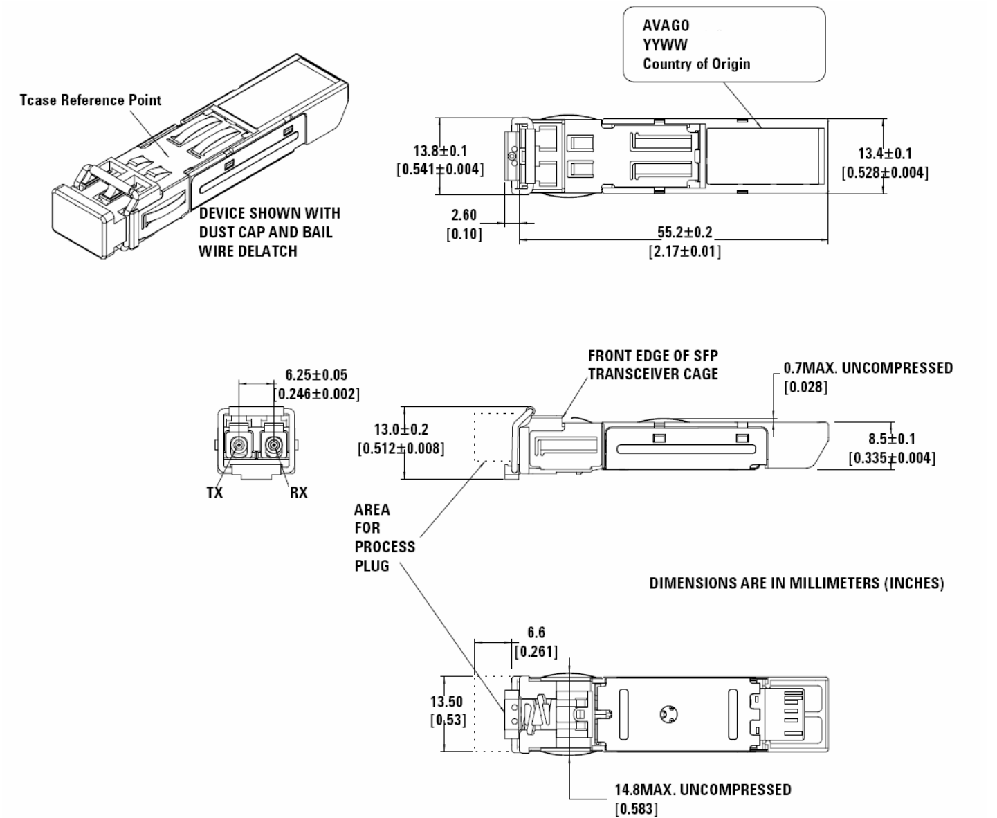
Figure 4: Mechanical Dimensions
