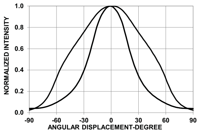
Figure 8: Radiation Pattern
