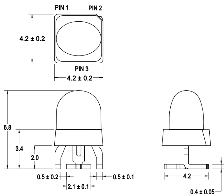
Figure 1: Package Drawing
