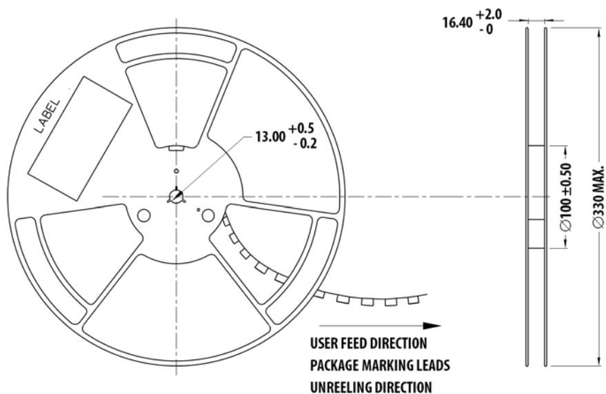
Figure 12: Reel Dimensions
