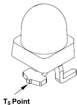
Figure 15: Solder Point Temperature on PCB
