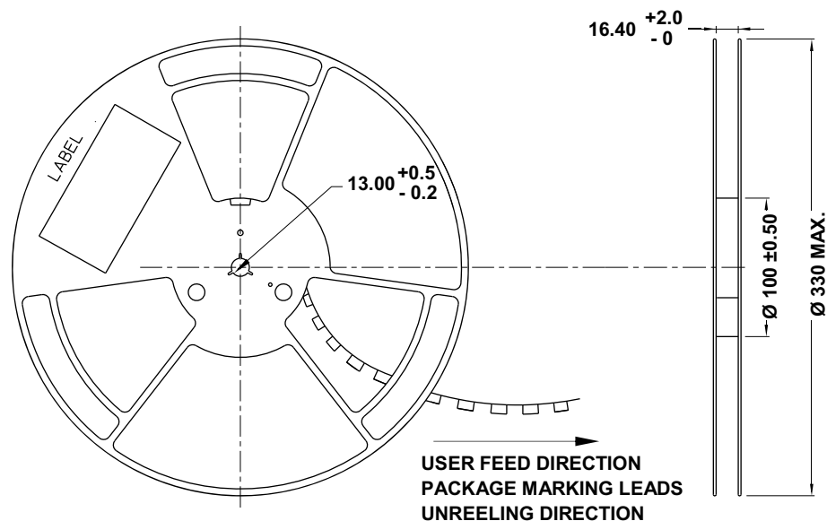
Figure 12: Reel Dimensions
