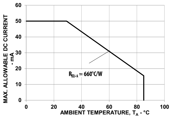
Figure 9: Maximum Forward Current vs. Ambient Temperature. Derate based on T_{J\text{ MAX}} = 110^{\circ}\text{C} .
