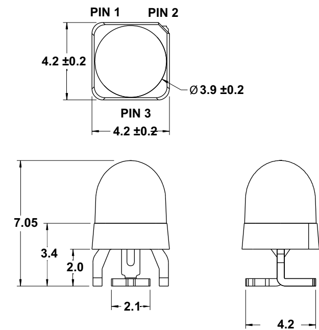
Figure 1: Package Drawing
