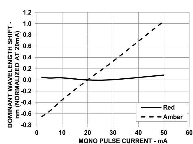
Figure 5: Dominant Wavelength Shift vs. Mono Pulse Current
