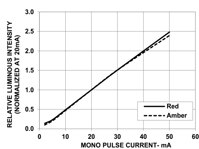
Figure 4: Relative Luminous Intensity vs. Mono Pulse Current
