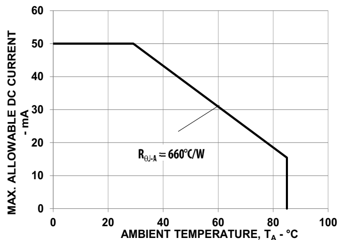
Figure 9: Maximum Forward Current vs. Ambient Temperature. Derate based on T_{J\text{ MAX}} = 110^{\circ}\text{C} .
