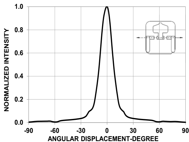
Figure 8: Radiation Pattern
