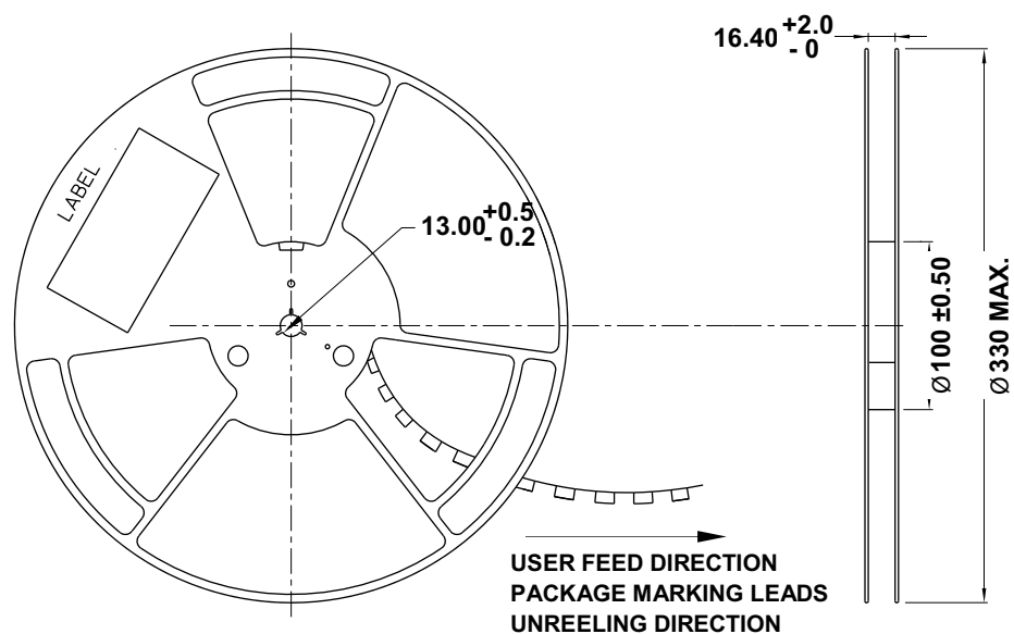
Figure 12: Reel Dimensions
