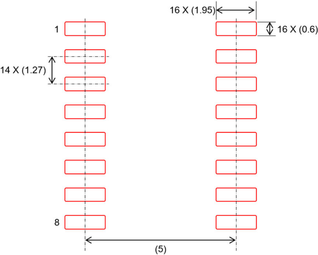
Figure 19: Recommended Land Pattern for TSSOP Package (in mm)
