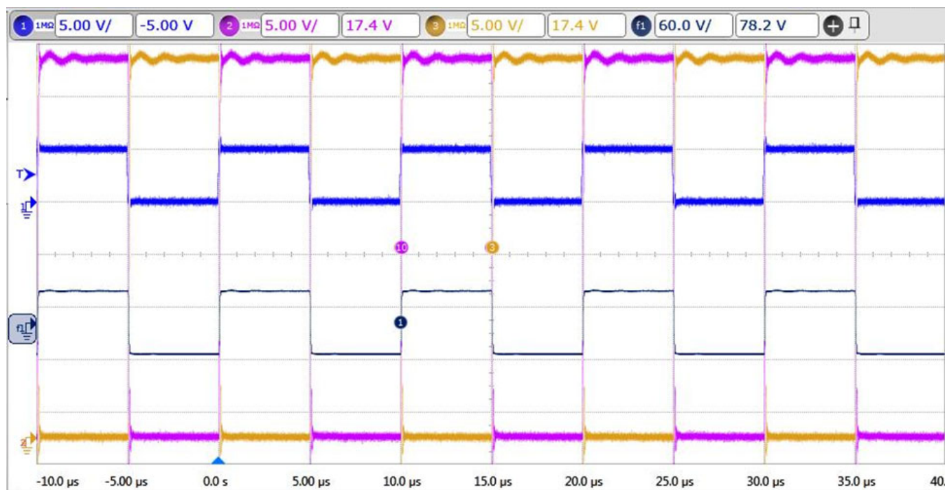
Figure 8: Example of Typical Line-End Signal with C_{load} = 100 pF, V_{DD} = 36 V, f_{OPERATE} = 100 kHz
