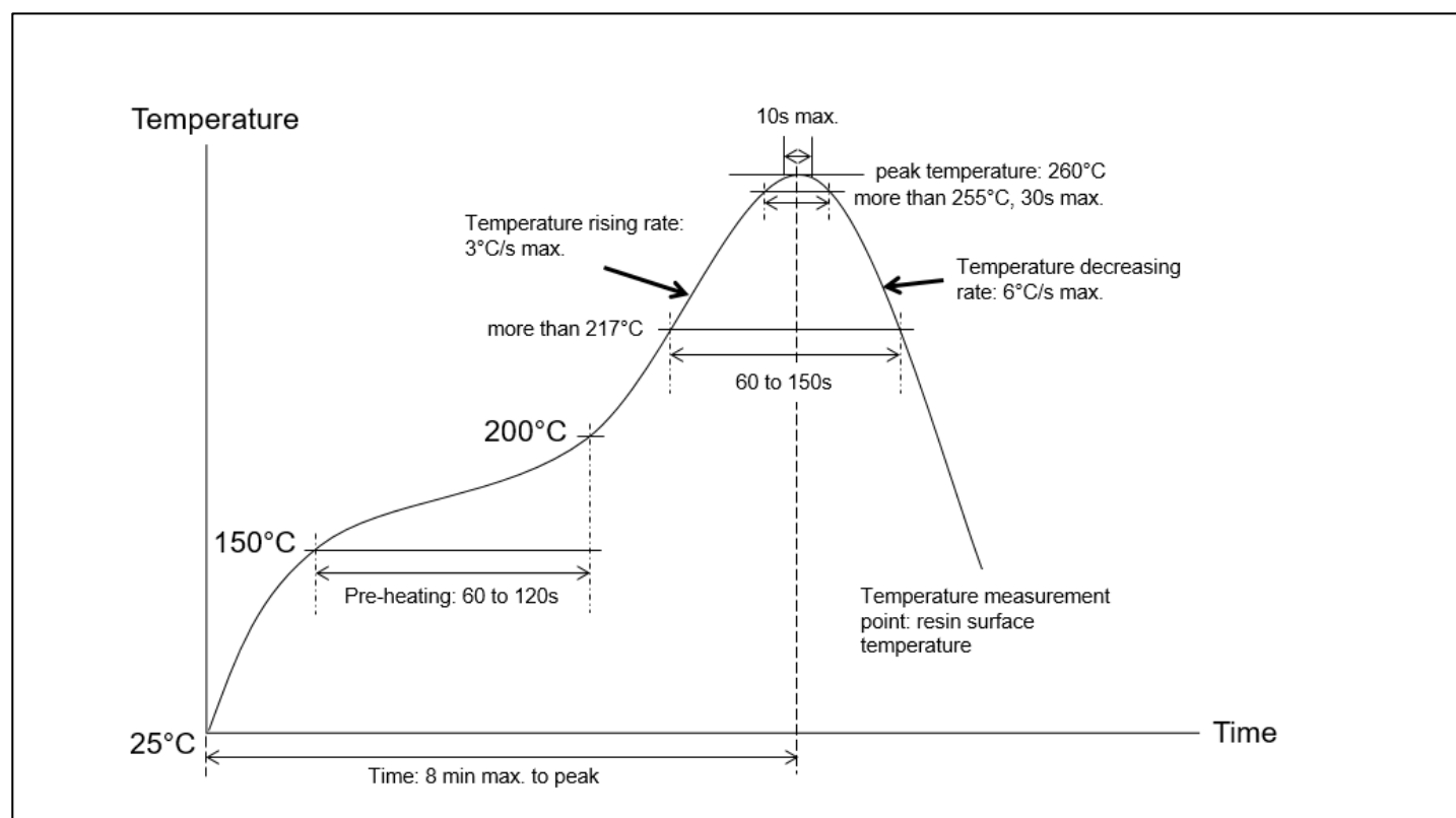
Figure 15: Typical Lead-Free Reflow Soldering Profile
