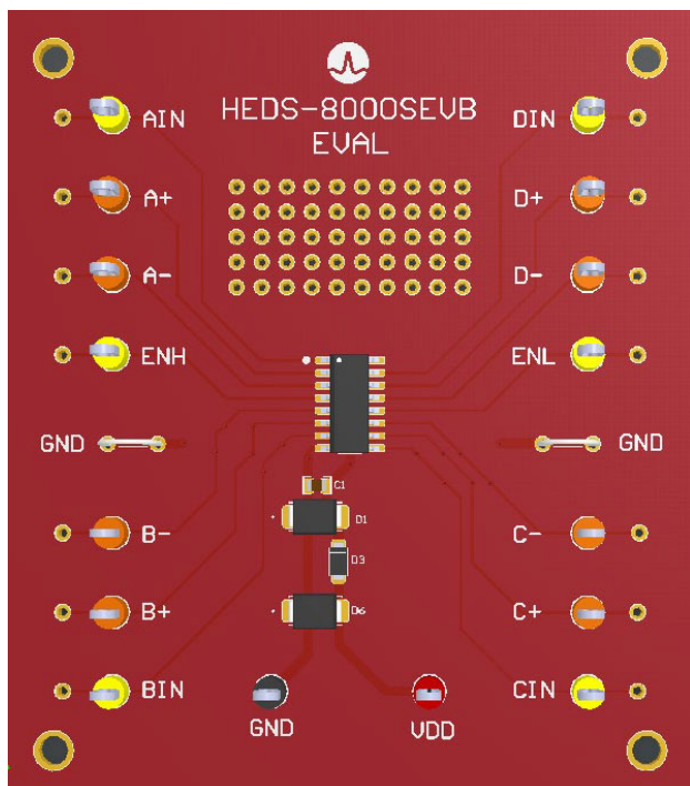
Figure 13: HEDS-8000SEVB Evaluation Board
