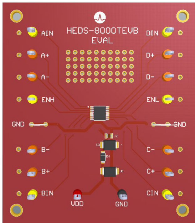
Figure 14: HEDS-8000TEVB Evaluation Board
