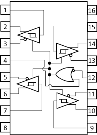
Figure 1: SOIC-16
