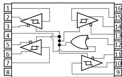
Figure 2: TSSOP-16
