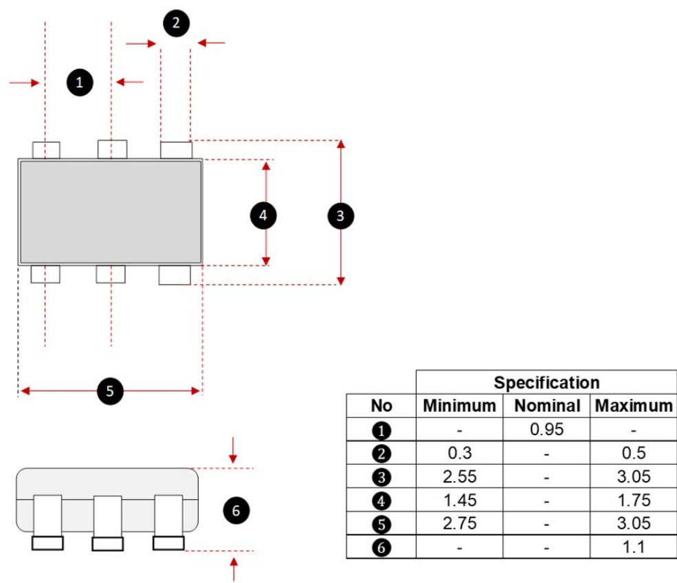
Figure 9: Package Dimensional Information
