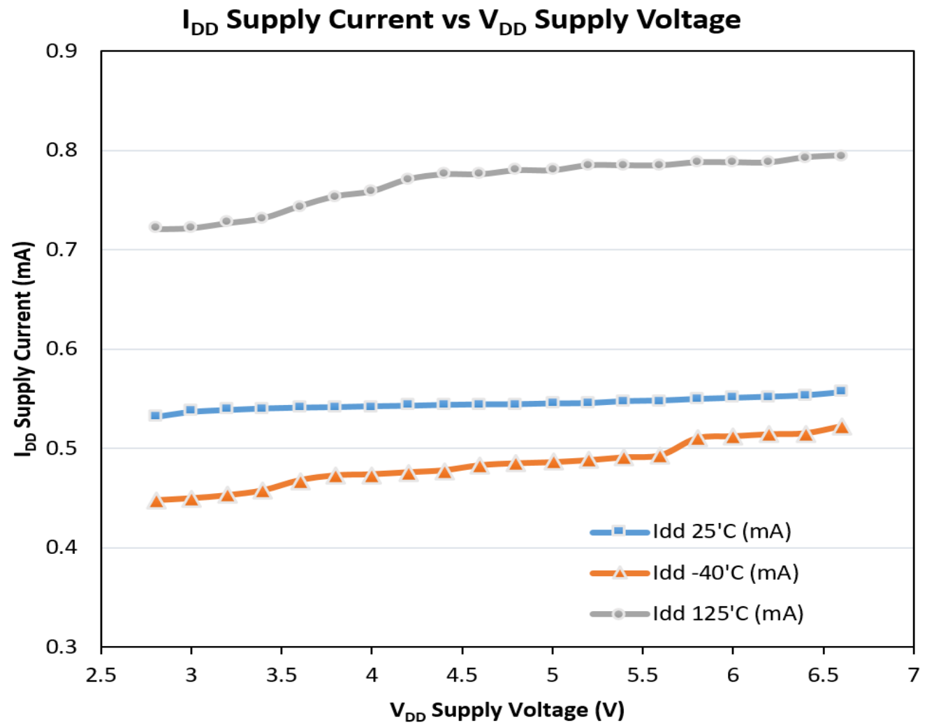
Figure 8: Supply Current
