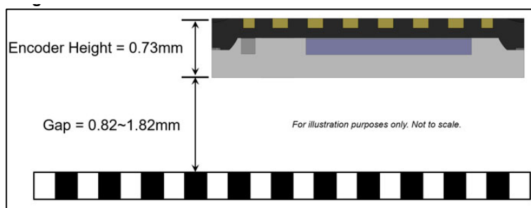
Figure 8: Encoder Placement Orientation
